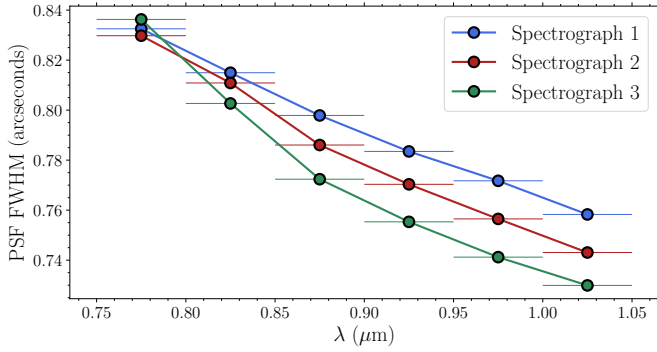
Figure A1. The average FWHM of the PSF as a function of wavelength and colour-coded by KMOS spectrograph. A two-dimensional image was created from each star observed during the K-CLASH survey by collapsing the full data-cube in a window of 0.05 \mu\text{m} in the wavelength direction. We then fit a two-dimensional Gaussian function to derive the FWHM of each observation, and average together all observations in the same spectrograph. This procedure is then repeated a further five times for increasing central wavelength. The FWHM of the PSF varies by around 0''.1 across the IZ spectral range, and by 0.03'' (at most) between spectrographs.
