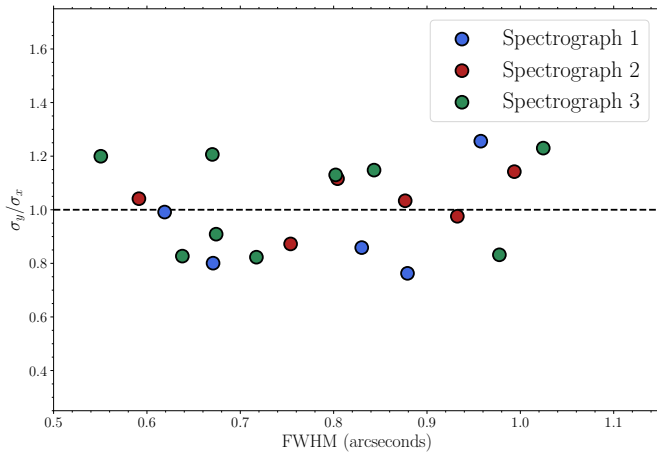
Figure A2. Ratio of the standard deviations ( \sigma_x and \sigma_y ) of the two-dimensional Gaussian fit to each star observed during the K-CLASH survey, plotted against the FWHM of the two-dimensional Gaussian fit. Points are colour-coded according to the KMOS spectrograph they were observed with. Each PSF is generally circular, with deviation from circularity at worst \approx 25\% .
