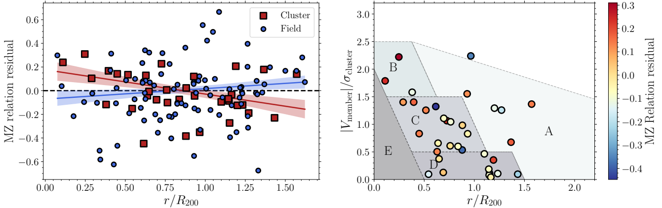
Figure 8. Correlation between a galaxy’s residual around the mass-metallicity relation and its location within its galaxy cluster. Left panel: we plot the MZ relation residuals against projected radii (scaled by the appropriate cluster R_{200} value) for the field (blue) and cluster (red) samples. There is no significant correlation between the MZ relation residuals and stellar mass or SFR for either sample. Right panel: for galaxies in the cluster sample, we show their locations in cluster phase-space. Each point is coloured by its residual around the MZ relation. We also use the simulations of Rhee et al. (2017) to show the regions in phase-space which roughly correspond to the locations where first infalling galaxies (A) and recent/intermediate infallers (B and C) reside. Region D is generally made up of a combination of intermediate and ancient infallers, as well as some “backsplash” galaxies, whilst E is dominated by ancient infallers. See Section 4.2 for details.
