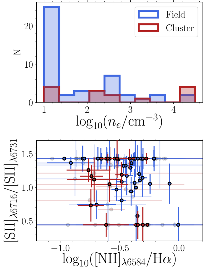
Figure 9. Top: A histogram of the electron number density in the mass-matched field (blue) and cluster (red) galaxy samples, estimated from the [\text{S II}]_{\lambda 6716}/[\text{S II}]_{\lambda 6731} line ratio and the calibration of Proxauf et al. (2014). Bottom: The [\text{S II}]_{\lambda 6716}/[\text{S II}]_{\lambda 6731} ratio against \log_{10}([\text{N II}]_{\lambda 6584}/\text{H}\alpha) . Each solid point has [\text{S II}] and [\text{N II}] S/N greater than 3, whilst faded points have S/N less than 3 in at least one line. We limit values of [\text{S II}]_{\lambda 6716}/[\text{S II}]_{\lambda 6731} to be between 0.44 and 1.44, the maximal values allowed by atomic physics.
