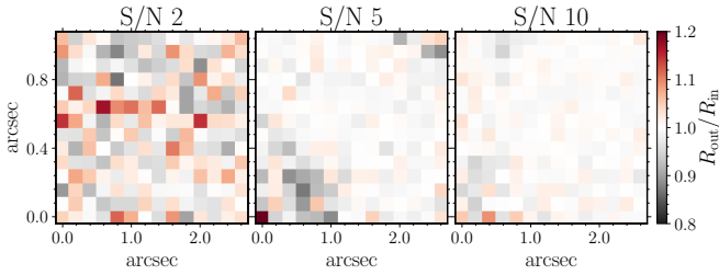
Figure B3. Recovering the H\alpha disc scale length ( R_{\text{disc}} ) of mock observations, for various locations on the IFU and S/N values. The model is a source with R_{\text{disc}} = 3 pixels, \epsilon = 0.2 and position angle 135^\circ .
