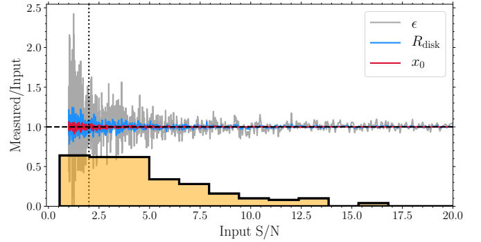
Figure B1. Recovery of the \text{H}\alpha profile parameters of mock observations, at various input S/N ratios of the \text{H}\alpha images. Note the image S/N value is the average S/N value of pixels within the best-fitting half-light radius. The dashed line represents an average image S/N of 2, and the histogram shows the S/N distribution of our observed \text{H}\alpha images described in Section 3.2. See Appendix B for details.
