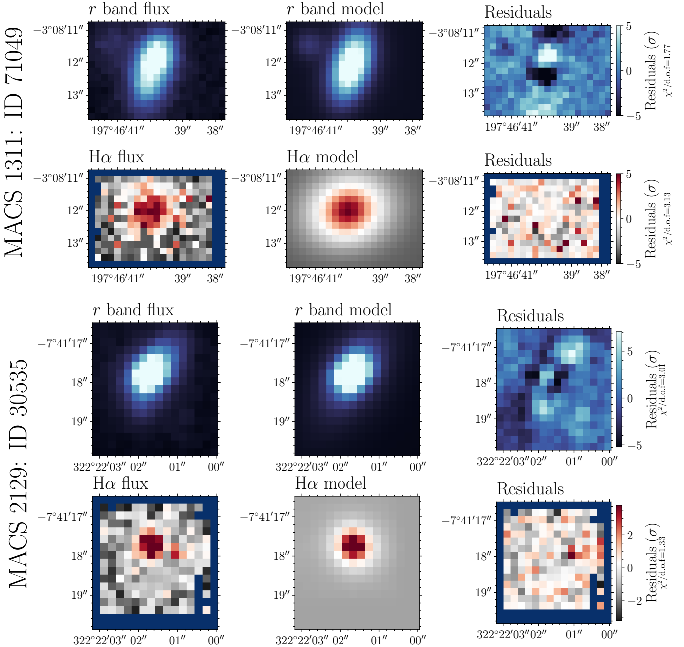
Figure 3. Postage-stamp images extracted from the R_c -band imaging (blue colour scales) and H \alpha emission maps (red colour scales) for two galaxies from our sample. The first column shows the data, the second shows the model and the third shows the residuals from the fit. Note that the R_c -band images have been shifted to match the centres of the H \alpha emission maps. The top object has an r_{e,\text{H}\alpha}/r_{e,R_c} markedly greater than unity (extended H \alpha emission compared to the stars), whilst the bottom panel shows an object with centrally concentrated H \alpha emission.
