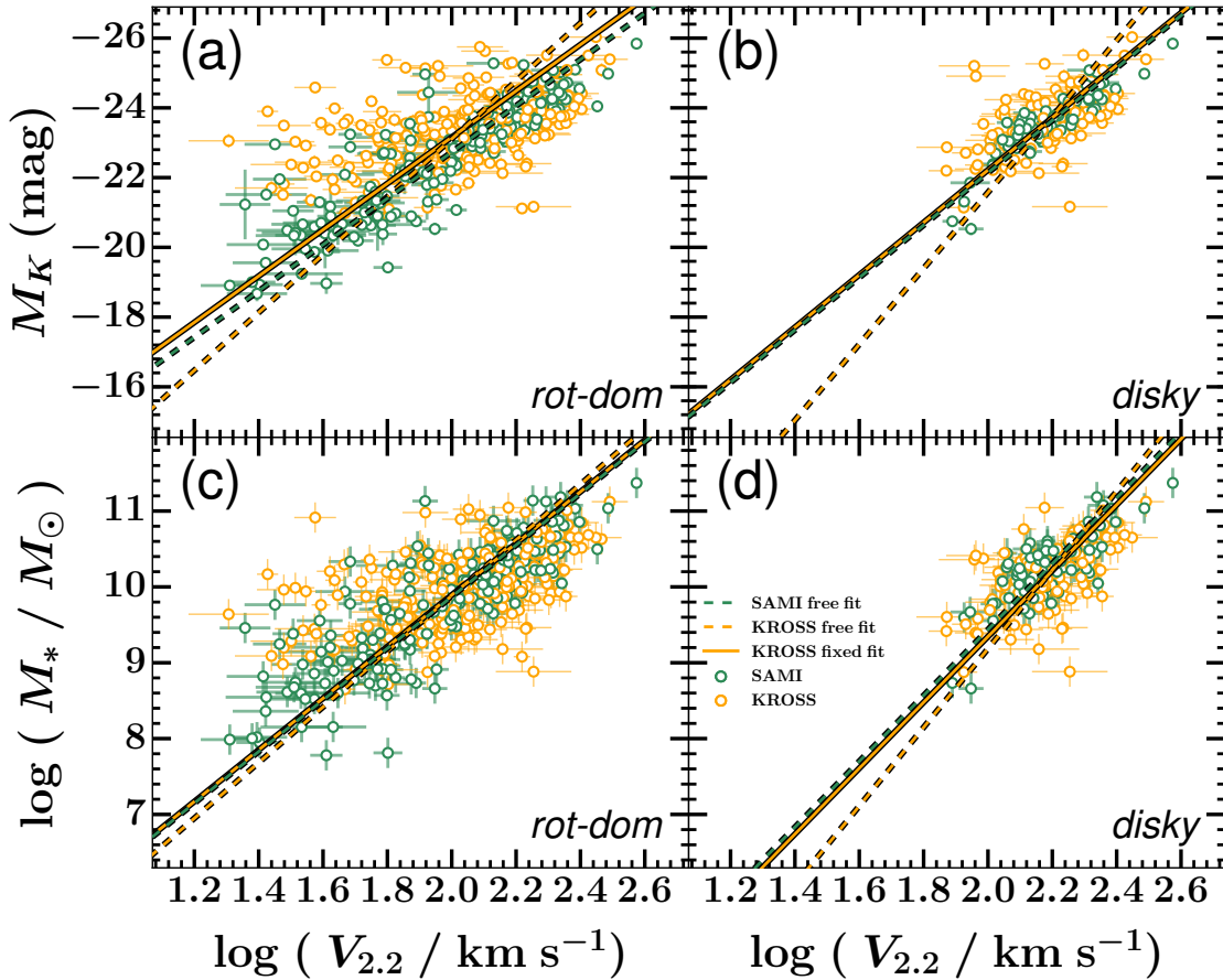
Figure 7. The M_K (top) and M_* (bottom) TFRs of the matched SAMI and KROSS rot-dom (left) and disky (right) sub-samples, as described in § 4. The dashed lines are the best fits with free slopes to each data set. The solid line in each panel is the best fit the KROSS TFR with the slope fixed to that of the best (free) fit to the corresponding matched SAMI TFR. There is no significant offset between the matched SAMI and KROSS M_K or M_* TFRs zero-points for the disky sub-samples that comprise disk-like galaxies that obey well the assumption of circular motion inherent in the TFR.
