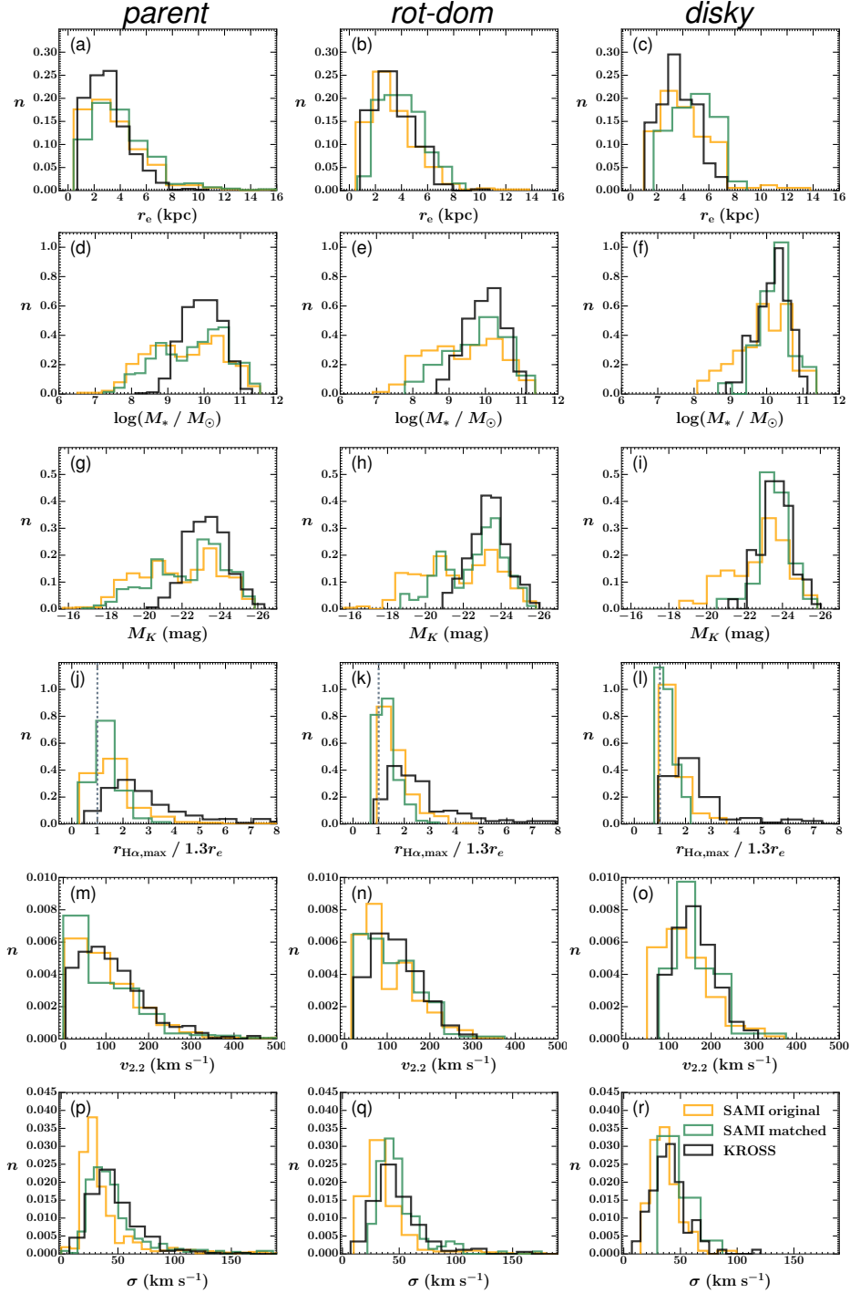
Figure 5. Distributions of r_e , M_* , M_K , r_{H\alpha,max}/1.3r_e , v_{2.2} and \sigma , as defined in the text, for respectively the original SAMI, matched SAMI and KROSS parent (left column), rot-dom (middle column) and disky (right column) sub-samples (defined in § 4). The dashed line in panels (j–l) indicates the radius at which we measure the rotation velocity for the TFRs shown in § 5.1 and § 5.2. By design, r_{H\alpha,max} \gtrsim 1.3r_e for the rot-dom and disky sub-samples of all three data sets. The same sub-sample selection criteria, when successively applied to both the original SAMI and matched SAMI data, tend to select larger, more massive, and more rapidly rotating galaxies from the latter data set than from the former. On average, the majority of KROSS galaxies are more massive, more rapidly rotating, and have more spatially extended H \alpha emission (relative to their size) than the majority of SAMI galaxies.
