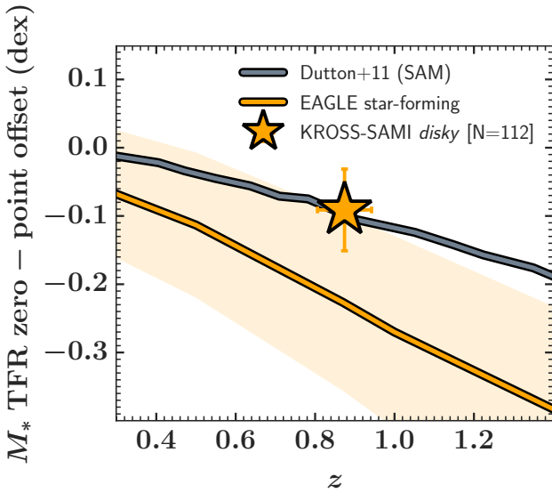
Figure 8. Evolution of the stellar mass TFR zero-point offset as a function of redshift (with respect to z \approx 0 ). We compare our measurement of the zero-point offset between z \approx 1 and z \approx 0 (from the KROSS-matched SAMI fixed slope comparison) to the zero-point evolution predicted by the semi-analytical modelling of Dutton et al. (2011) and star-forming model galaxies in the EAGLE simulation (Schaye et al. 2015; Crain et al. 2015; McAlpine et al. 2015). We linearly interpolate between each point to better highlight the predicted trends as a function of redshift. The shaded orange region indicates the root-mean-square scatter of the star-forming model EAGLE galaxies at each redshift, again linearly interpolated to highlight the trend with redshift. Our measure of the TFR zero-point evolution since z \approx 1 for disky galaxies agrees well with the prediction from Dutton et al. (2011), but is also consistent with the zero-point evolution seen for the model EAGLE galaxies.
