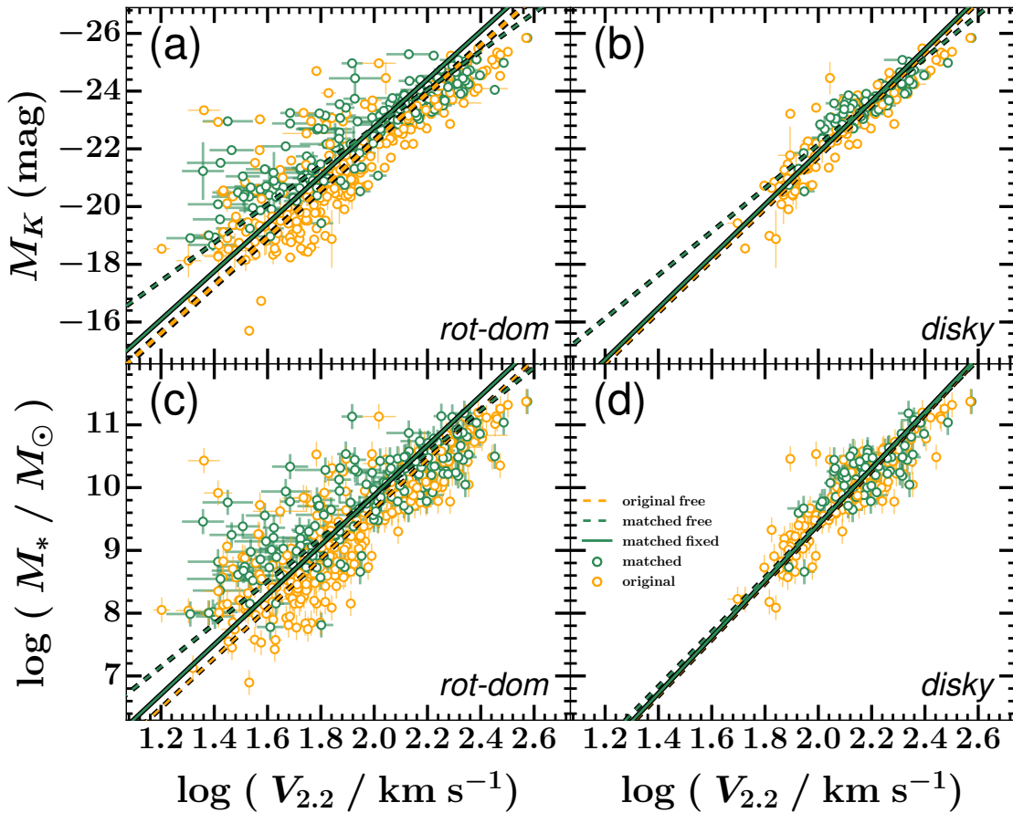
Figure 6. The M_K (top) and M_* (bottom) TFRs for the original SAMI and matched SAMI rot-dom (left) and disky (right) sub-samples, as described in § 4. In each panel the dashed lines are the best fits with free slopes to each data set. The solid line is the best straight line fit to the matched SAMI data with the slope fixed to that of the best free fit slope to the corresponding original data. In all cases the best free fit slope for the matched SAMI TFR is shallower than the best fit slope for the corresponding original SAMI relation. For a fixed slope the zero-point of the TFR in each case differs between the original SAMI and matched SAMI data, although this difference is not significant between the disky sub-samples.
