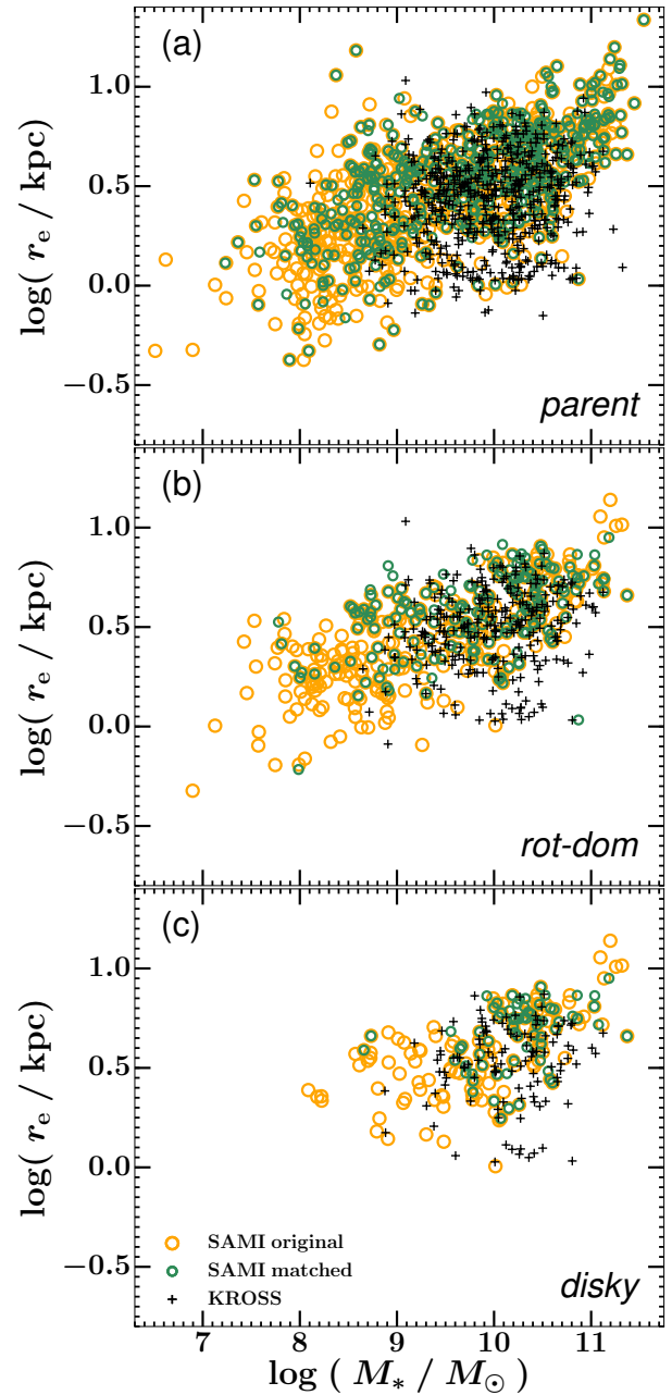
Figure 3. Mass-size relation of the original SAMI, matched SAMI, and KROSS parent (panel a), rot-dom (panel b) and diskly (panel c) sub-samples. Sizes are measured from stellar continuum light in broadband images (in the restframe r -band ( \sim 0.6\mu\text{m} ) for SAMI galaxies, and restframe i -band ( \sim 0.8\mu\text{m} ) for KROSS galaxies). Error bars are omitted for clarity. In each panel, the three data sets generally follow the same trend, more massive galaxies being larger (as expected). The KROSS sub-samples, however, are limited to higher stellar masses than the original SAMI and matched SAMI sub-samples.
