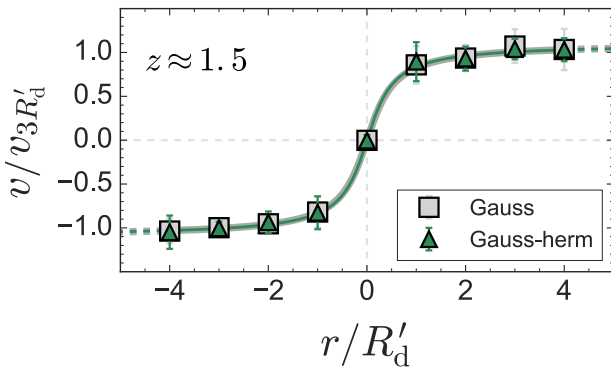
Figure A3. The median-average of the individual stellar-scaled rotation curves for our z \approx 1.5 galaxy sample, extracted from velocity maps derived from either Gaussian triplet or Gaussian-hermite triplet fits to the emission lines in each of the data cubes. The average curves include those galaxies with sufficient pixels in both the Gaussian- and Gaussian-hermite-derived velocity maps to reliably measure a rotation velocity from both. The two curves are in good agreement, with no significant deviations in the range \pm 4R'_d .
