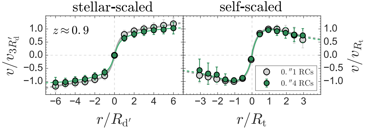
Figure A4. The median-average z \approx 0.9 (KROSS) stellar-scaled rotation curve (left panel) and the corresponding self-scaled curve (right panel) constructed from individual galaxy rotation curves extracted from velocity maps (as described in § 3.3) sampled with either 0.''1 or 0.''4 spaxels. The two different samplings result in curves that are in good agreement, within uncertainties, although the average of the 0.''4 -sampled stellar-scaled curves is slightly shallower than the corresponding 0.''1 -sampled average curve. Most importantly, for either choice of spatial sampling, we draw the same conclusion - that the shape of the median average rotation curve for the same galaxies starkly differs depending on the normalisation technique.
