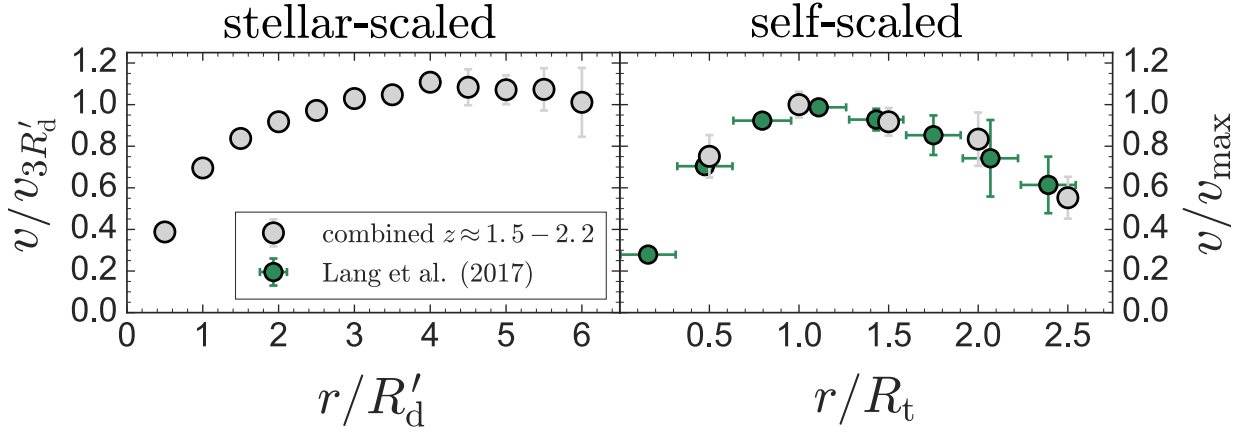
Figure A6. A demonstration of our ability to recover a declining rotation curve from stacked position-velocity diagrams adopting the self-scaled ( R_t, v_{\max} ) normalisation prescription of Lang et al. (2017). The grey points represent the median rotation curve extracted from the stacked position-velocity diagrams of the combined z \approx 1.5 and z \approx 2.2 KMOS samples. This combined sub-sample is designed to be large enough to reduce the effects of noise in the resultant average rotation curve whilst also comprising those galaxies best matched in redshift to the stacking sample in Lang et al. (2017). The median stellar mass of the combined sample is \log M_*/M_\odot = 10.3 \pm 0.3 , where the uncertainty is the median absolute deviation from the median. The green points represent the average rotation curve as constructed by Lang et al. (2017) and presented in Figure 5 of that work. Left: The stellar-scaled rotation curve for the combined z \approx 1.5 and z \approx 2.2 KMOS samples remains flat . Right: The two self-scaled curves exhibit the same shape, including a strong decline in velocity at large fractional radii. For the same galaxies (i.e. the grey points in each panel), the rotation curve either remains flat (stellar-scaled) or turns over (self-scaled), depending on the normalisation prescription.
