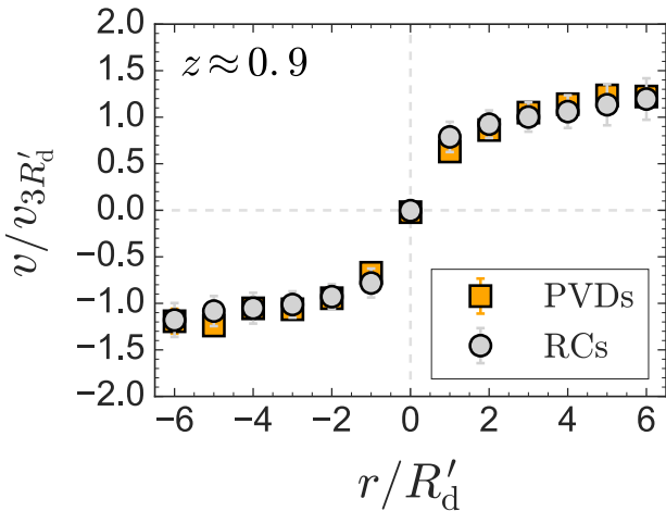
Figure A5. A comparison between the median-average of the individual z \approx 0.9 (KROSS) stellar-scaled rotation curves (grey points; see § 4.1) and the corresponding rotation curve for the same galaxies derived from stacked galaxy H \alpha emission using the method outlined in § 4.2. The two curves are in good agreement, within uncertainties (despite the latter rising slightly more slowly in its inner regions than the former) thus verifying the validity of our methods.
