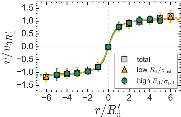
Figure A1. A comparison between the median-average z \approx 0.9 (KROSS) stellar-scaled rotation curve constructed from individual galaxy rotation curves for respectively the total KROSS sample, those KROSS galaxies that are smallest compared to the size of the PSF (defined as those with a ratio R_d/\sigma_{\text{psf}} lower than the 30 th percentile of the total distribution for KROSS galaxies), and those KROSS galaxies that are largest compared to the size of the PSF (defined as those with a ratio R_d/\sigma_{\text{psf}} larger than the 60 th percentile of the total distribution for KROSS galaxies). The corresponding best fit model (see § 4.2.4) to each rotation curve is also displayed as a solid line (dashed where extrapolated beyond the measurements). The shapes of the three curves are in good agreement with no significant deviations between the three. The ratio of the galaxy size to the size of the PSF has no significant impact on the shape of the average stellar-scaled KROSS rotation curve.
