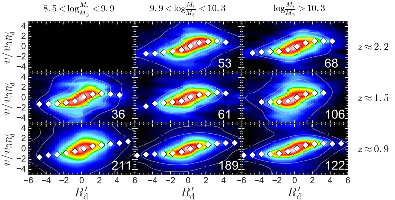
Figure A7. Median-averaged normalised position-velocity diagrams for samples of galaxies from our analysis separated in to bins of redshift and mass. The position-velocity diagrams are derived from stacked H \alpha emission. We overlay grey contours corresponding to a signal-to-noise ratio of 5 and 10. The white diamonds in each panel represent the peak position of the best fit to the spectrum corresponding that radial column. The majority of the curves remain flat or continue to rise out to large radii.
