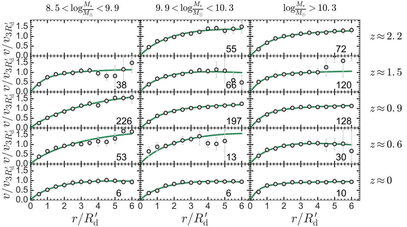
Figure 7. Average wrapped, normalised rotation curves for samples of galaxies from our analysis separated into bins of redshift and mass. The rotation curves were constructed in the same manner as for Figure 6. The green solid line in each panel represents the best fit model curve. The shape of each rotation curve is consistent, within uncertainties, with remaining flat or continuing to rise out to large radii.
