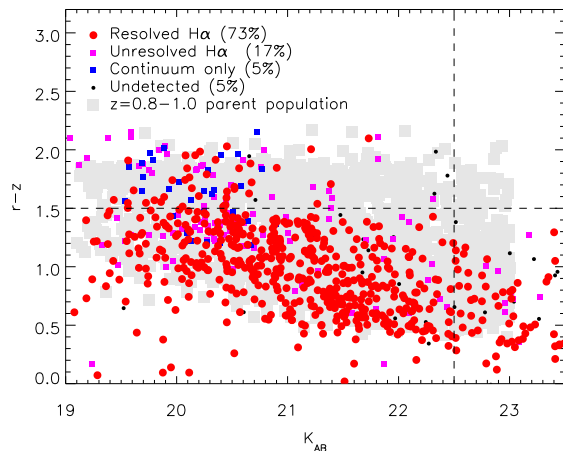
Figure 2. The r - z vs. K colour magnitude diagram for the KROSS sample. The red points are galaxies for which we resolved the H\alpha emission. The magenta squares are those galaxies in which we detect H\alpha ( > 5\sigma ) but it is not spatially resolved and the blue squares are those where we detect continuum only. The small number of black points are those galaxies which are undetected in our spectra. The background region composed of light grey squares shows the position of the z = 0.8 - 1.0 galaxy population from the VIDEO survey (Jarvis et al. 2013), demonstrating that the KROSS galaxies are typical of the parent star-forming population.
