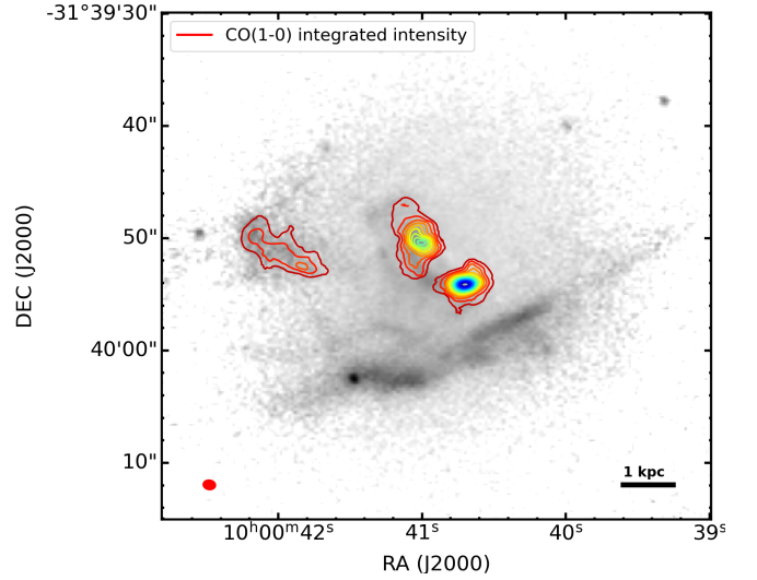
Figure 11. CO(1-0) integrated intensity contours overlaid to the B-I dust extinction map of NGC 3100 (see Paper I) zoomed in the central 50'' \times 50'' ( \sim 9 \times 9 \text{ kpc}^2 ). CO contours are drawn at 1, 3, 9...times the 3\sigma rms noise level. The CO beam size and scale bar are shown in the bottom-left and bottom-right corners, respectively; East is to the left and North to the top.
