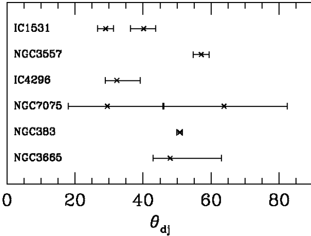
Figure 4. Distribution of intrinsic jet-disc orientation angles, \theta_{\text{dj}} from Table 4. For IC 1531 and NGC 7075, the disc orientation is ambiguous and both possible values are plotted.
