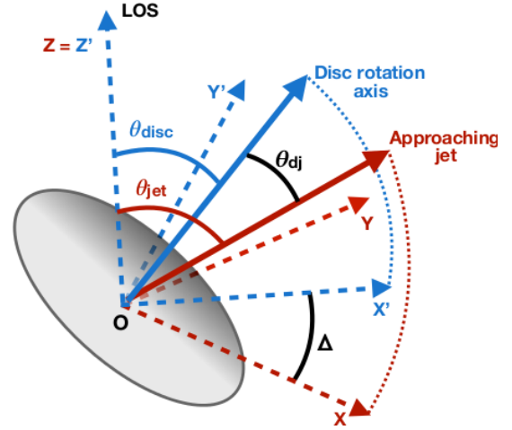
Figure A1. Sketch describing the 3D geometry of the jet-disc system for an illustrative case. The Cartesian system Oxyz is built so that the origin is in the core, the z axis is along the line of sight (positive sign towards the observer), and the x - y axes are in the plane of the sky. The x axis is parallel to the projection of the jet (positive sign along the projection of the approaching jet, indicated as a solid red arrow). The angle between the approaching jet and the line of sight is \theta_{\text{jet}} . Similarly, in the Ox'y'z' Cartesian system, the origin is in the core, the z' axis is again along the line of sight, the x' - y' axes are in the plane of the sky, and x' lies along the projection of the disc rotation axis (i.e. the vector normal to the disc plane, indicated as a solid blue arrow). The inclination of the gas disc to the line of sight is given by the angle \theta_{\text{disc}} . \theta_{\text{dj}} is the angle between the jet and the disc rotation axes and defines the intrinsic relative orientation of the CO disc and the radio jets. The projected jet-disc relative orientation is given by the angle \Delta . The grey ellipse illustrates the CO disc, a darker grey shade is used to indicate the near side of the disc. See the text for details.
