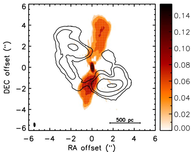
Figure 5. Masked JVLA continuum map of NGC 3100 at 10 GHz with ALMA CO integrated intensity contours superimposed in black. CO contours are drawn at 9, 27, 81 and 180 times the 1\sigma rms noise level ( 1\sigma = 0.6 mJy beam ^{-1} ; see Paper I). The beam and the physical scale bars are drawn in the bottom-left and bottom-right corners, respectively. The wedge on the right shows the colour scale in Jy beam ^{-1} .
