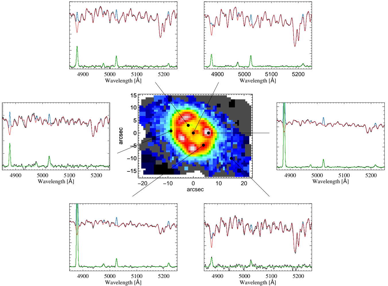
Figure 3. Fits of the SAURON spectra of NGC 4314. The inset corresponds to the H \beta flux map (see also Fig. 5j). Data bins with A/N values below 5 (see 3.2) are displayed in the different maps as dark grey. Six spectra and their corresponding fits at different locations are shown around the inset image. In each panel the black line shows the galaxy spectrum, the red line is the best fitting stellar template, and the blue line is the best fit when emission lines are added. Below each spectrum the differences between the galaxy spectrum and the best stellar template are shown in black. The emission-line fits are overlaid in green. The spectra have been arbitrarily shifted in the vertical direction for presentation purposes.
