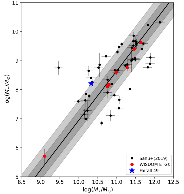
Figure 9. The location of Fairall 49 (blue star) on the M_{\bullet} - M_{\star} relation. Black and red dots show ETGs from Sahu et al. (2019) and the WISDOM papers, respectively. The solid line shows a fit using BayesLineFit (Lelli et al. 2019); the light and dark grey bands correspond to 1 and 2 times the orthogonal intrinsic scatter in the relation.
