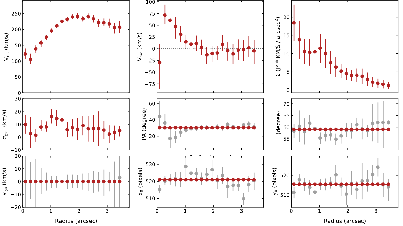
Figure 4. Best-fit parameters from 3\text{D}\text{BAROLO} . From top to bottom, from left to right: rotation velocity, radial velocity, surface brightness profile, velocity dispersion profile, position angle, inclination angle, systemic velocity, coordinates of the kinematic center. Grey points show initial estimates from a first fit in which all parameters are free, while red points show final estimates from a second fit in which i , PA, V_{\text{sys}} , x_0 and y_0 are fixed to the mean value across the rings.
