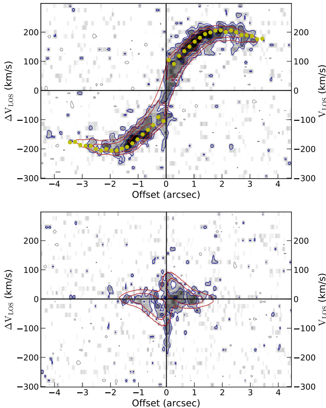
Figure 6. Position-velocity diagrams along the major (top) and minor (bottom) axes of the CO disk (see dashed lines in Figure 3). Positive and negative velocities correspond to the North-Eastern and South-Western sides of the disk, respectively (see Fig. 5)
