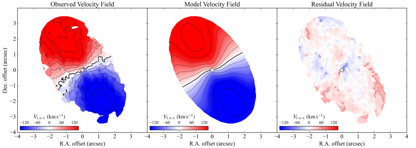
Figure 5. Velocity fields from the observed cube (left panel), model cube (middle panel) and residual cube (right panel). The velocity fields are cropped beyond R \approx 3.5'' because we do not model the kinematics at larger radii. In the left and middle panels, the velocity contours range from \pm 240 \text{ km s}^{-1} in steps of 30 \text{ km s}^{-1} (twice the channel width). In the right panel, the velocity contours are at \pm 30 \text{ km s}^{-1} . In all panels, the white star corresponds to the dynamical center.
