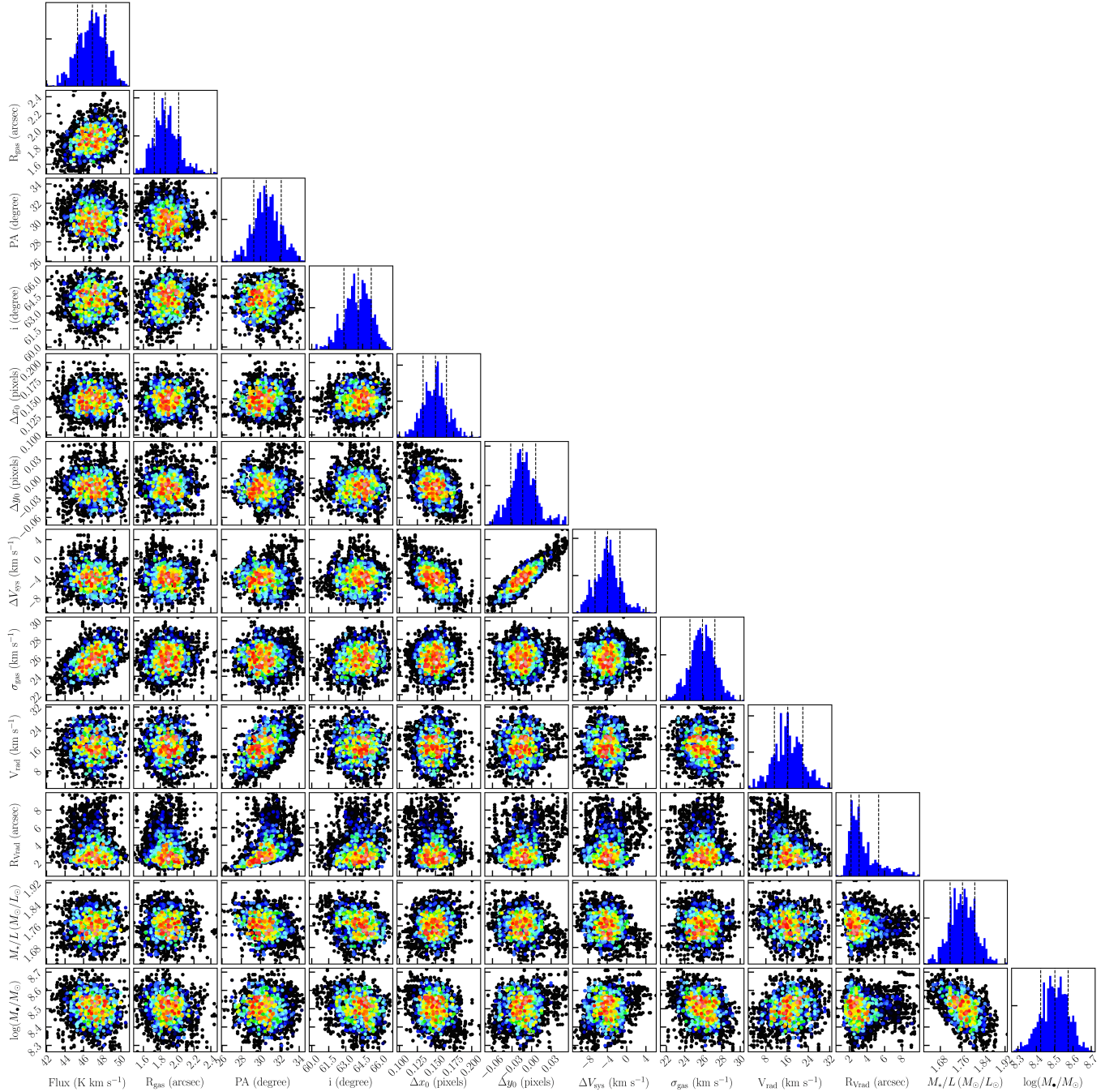
Figure 8. Posterior probability distributions of fitting parameters from the forward modeling with KINMS . In the marginalized 1D distributions, the dashed lines correspond to the 0.16, 0.50, and 0.84 quantiles ( 1\sigma confidence intervals). In the 2D distributions, the rainbow colours indicate the maximum likelihood for a given combination of two parameters, with white corresponding to the maximum likelihood and dark blue to a 3\sigma confidence level.
