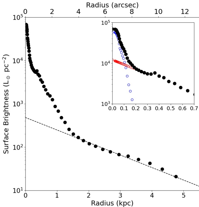
Figure 2. Surface brightness profile of Fairall 49 from the HST/WFPC2 image in the F606W filter. The dashed line shows an exponential fit to the outer parts. The inset zooms at small radii ( R < 0.7 kpc): the blue circles corresponds to the inner HSB component that is likely dominated by the AGN and/or starburst emission, the red circles shows the inward exponential extrapolation of the stellar component. See text for details.
