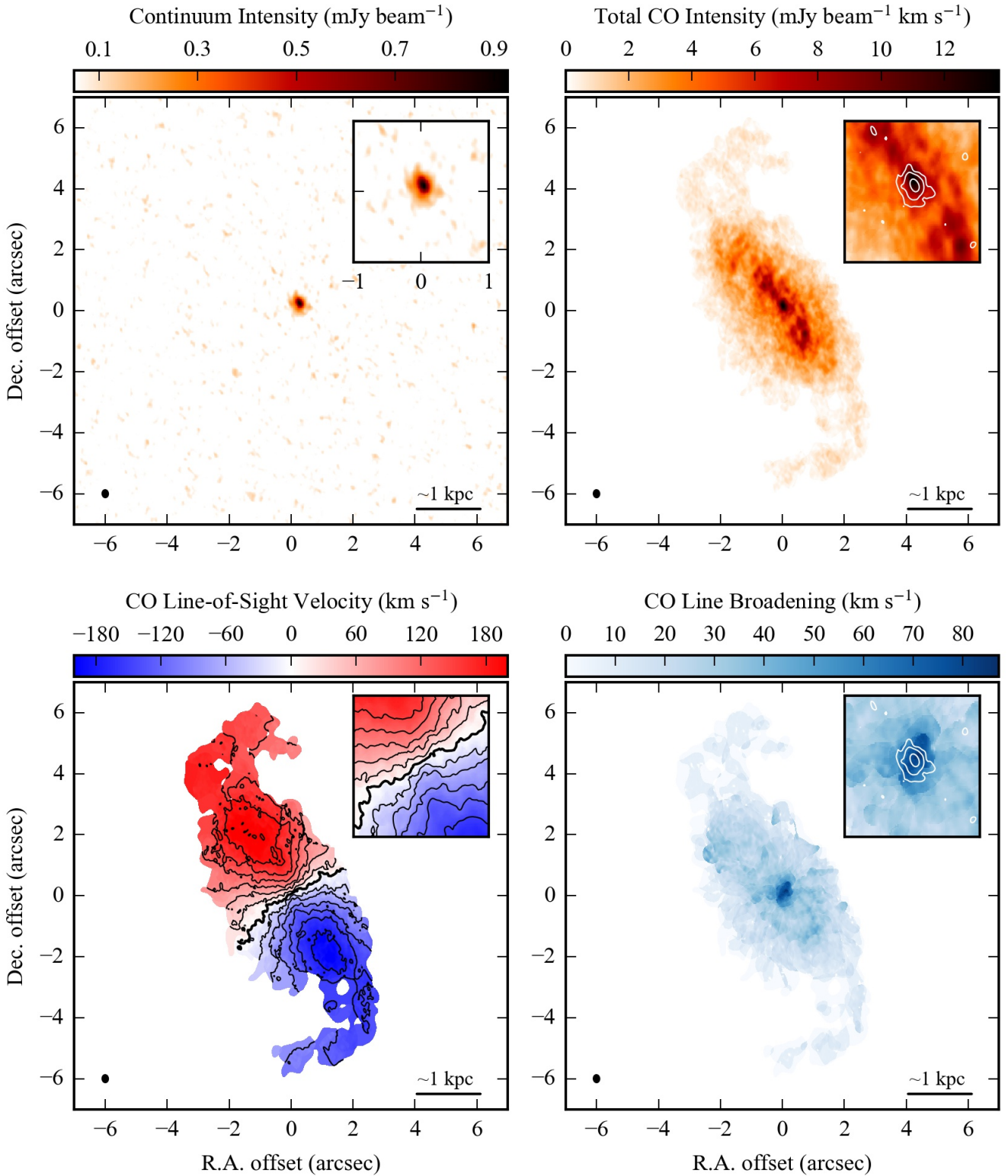
Figure 3. Overview of ALMA observations: 1.3 mm continuum map (top-left panel), CO moment-zero map (top-right panel), CO moment-one (bottom-left panel), and CO moment-two map (bottom-right panel). In all panels, the ellipse in the bottom-left corner shows the synthesized beam, while the bar in the bottom-right corner corresponds to \sim 1 \text{ kpc} . The insets zoom into the central 2'' \times 2'' area; the moment-zero and moment-two maps are overlaid with the 1.3 mm continuum emission (white contours at 3\sigma , 6\sigma , and 12\sigma ). In the moment-one map, iso-velocity contours range from \pm 240 \text{ km s}^{-1} in steps of 30 \text{ km s}^{-1} (twice the channel width); the bold contour corresponds to the systemic velocity (set to zero).
