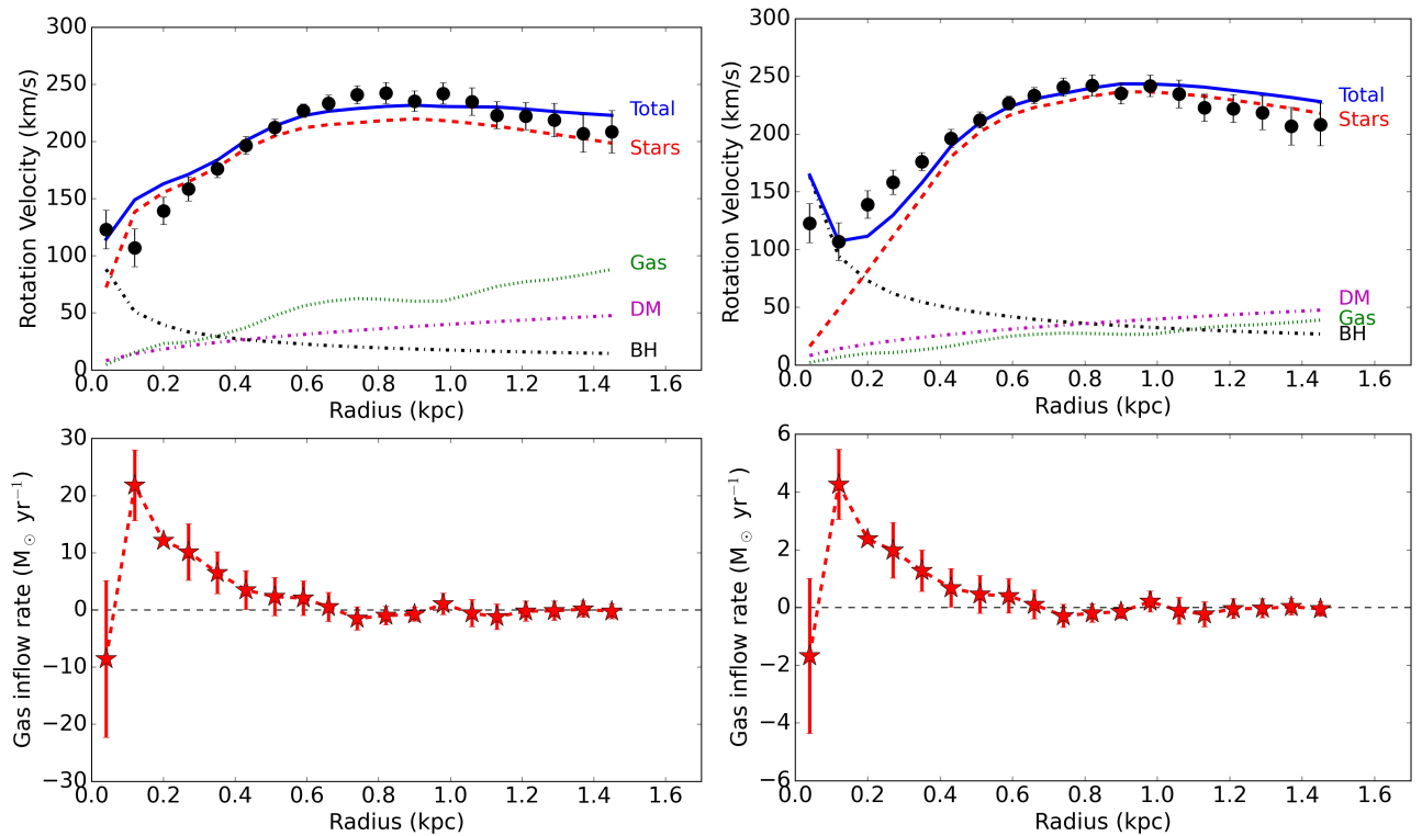
Figure A2. Same as Figure 7 but calculating the stellar gravitational contribution with no HSB subtraction (left panel) and maximal HSB subtraction (right panel). Both mass models do not provide a good fit to the inner rotation curve and are probably unphysical, but can be used to estimate systematic uncertainties on the SMBH mass and gas inflow rate.
