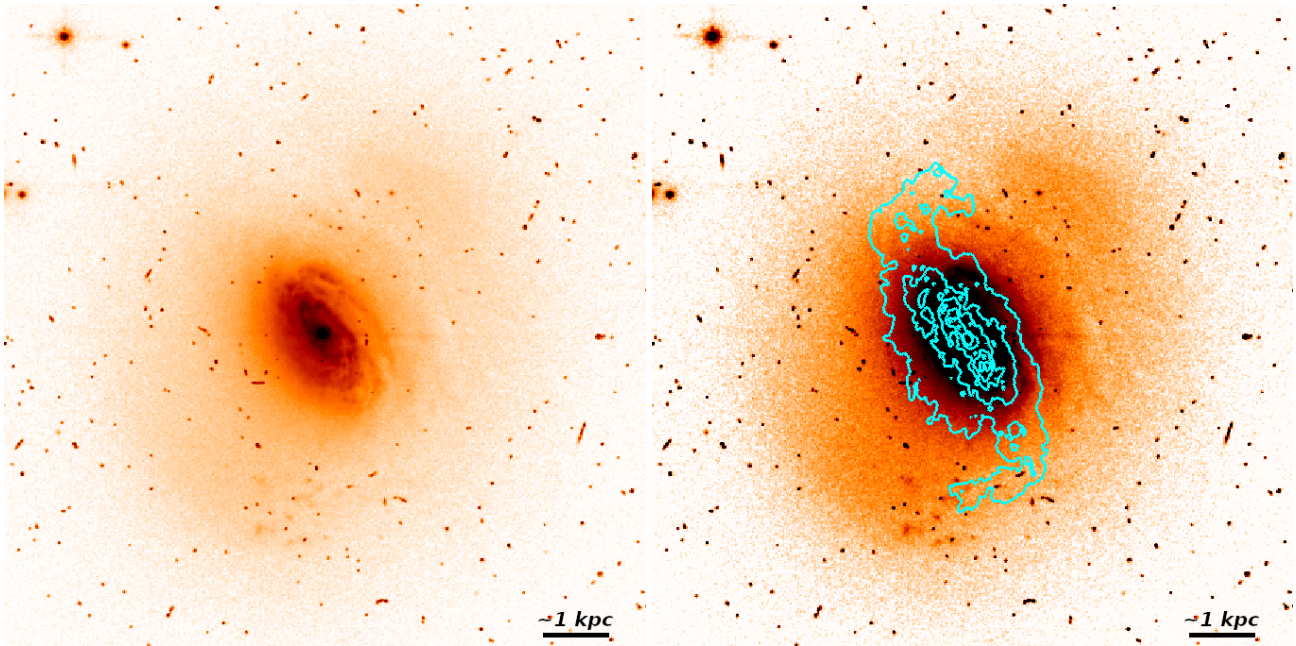
Figure 1. HST/WFPC2 image of Fairall 49 in the F606W filter. The two panels show the same HST image but use a different color stretching to highlight different features in the galaxy. The left panel shows the inner spiral disk, while the right panel highlights the outer asymmetric stellar distribution superimposed with the CO(2-1) emission (cyan contours). Contours increase from 0.14 ( \sim 3\sigma ) to 8 mJy beam ^{-1} km s ^{-1} . The bar to the bottom-right corner equals \sim 2.5'' , corresponding to \sim 1 kpc for the assumed distance of 86.7 Mpc. North is up; East is left.
