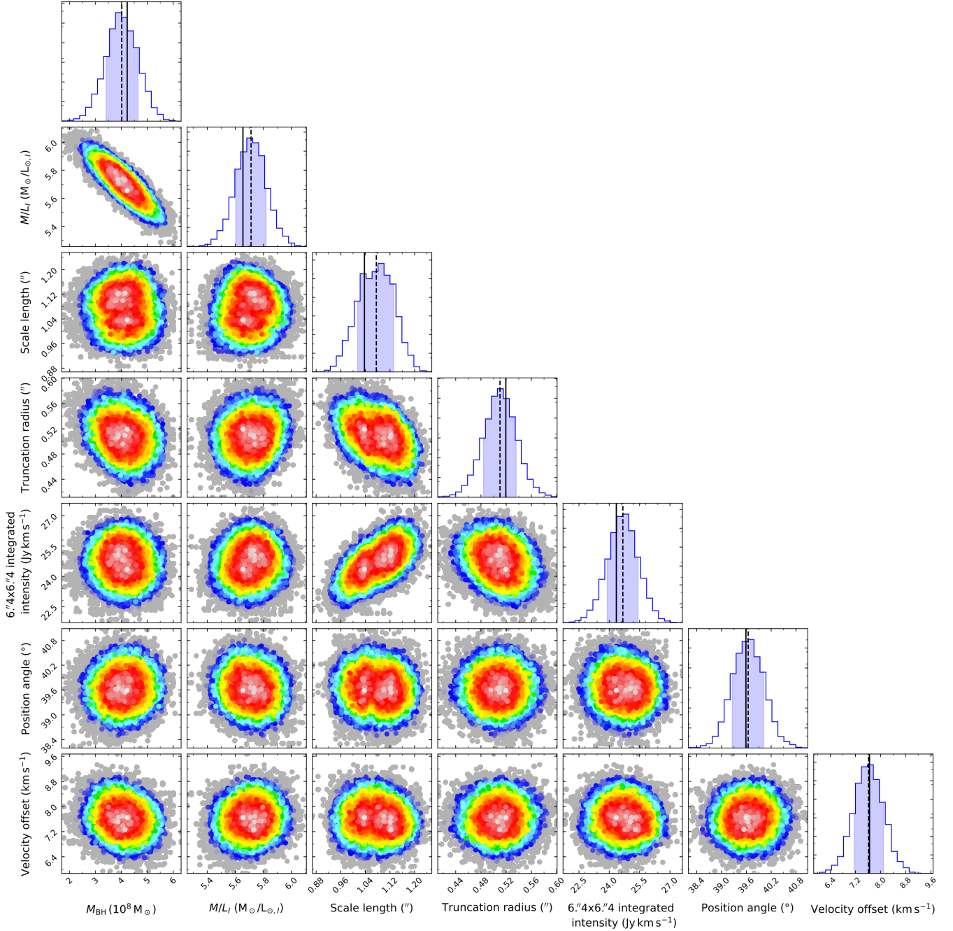
Figure 4. Corner plots showing the covariances between all model parameters, from an MCMC fit at fixed inclination. Each point is a realisation of our model, colour-coded to show the relative log-likelihood of that realisation, with white points the most likely and blue least. Grey points are realisations with \Delta\chi^2 > \sqrt{2N} relative to the best-fitting model, and are even less likely. The only significant covariance is between the SMBH mass and the mass-to-light ratio, that corresponds to attributing the dynamical mass across the SMBH and stellar distribution. The weak covariances between integrated intensity, scale length and truncation radius are due to the integrated intensity being the normalisation of the surface brightness profile, and therefore dependent on the exact fits. Histograms show 1D marginalisations of each parameter, with black lines denoting the median (dashed) and best-fitting (solid) values. We note that the asymmetry of the posterior means that the most likely value and median are very slightly different. The shaded region indicates the 68% confidence interval.
