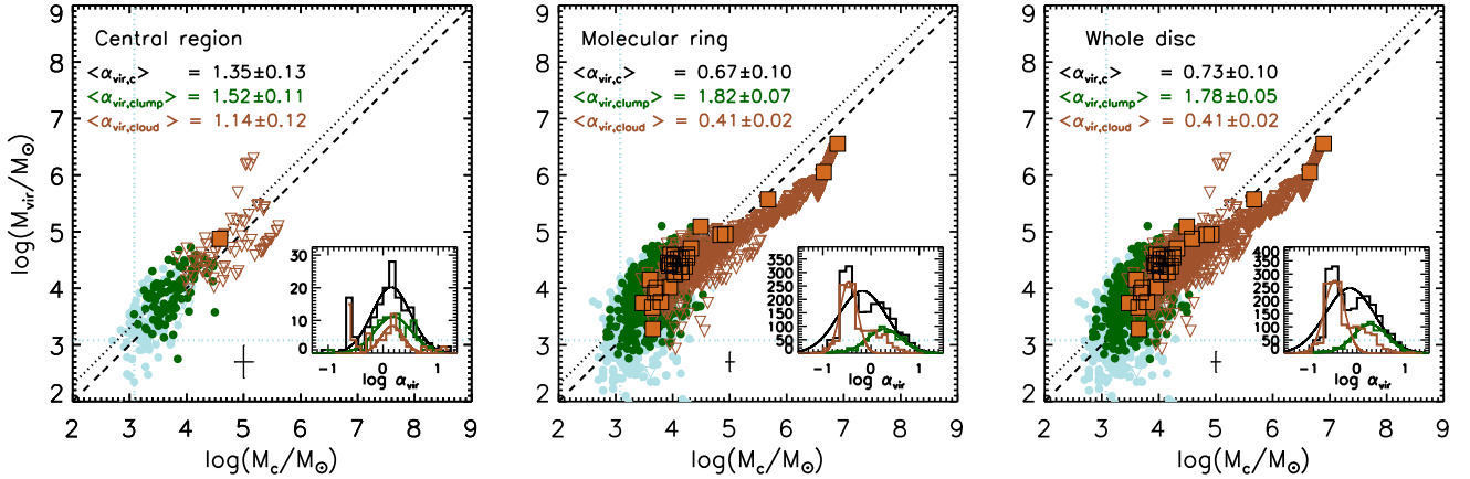
Figure 6. Virial mass – gaseous mass relation of molecular structures in the central region, molecular ring and whole disc of NGC 404, respectively. Symbols are as for Fig. 4. The black dashed lines show the 1 : 1 relations (i.e. \alpha_{\text{vir},c} = 1 ) and the black dotted lines the 2 : 1 relations (i.e. \alpha_{\text{vir},c} = 2 ). The vertical and horizontal blue dotted lines indicate our mass detection limit ( \log(10\delta_M/M_{\odot}) = 3.08 ; see Section 3.1). In the inset of each panel, the distributions of \log \alpha_{\text{vir},c} of all resolved molecular structures (black), clumps (green) and clouds (brown) are shown, with their best log-normal fits overlaid in matching colours. The corresponding mean virial parameters are listed in the legend.
