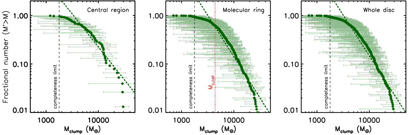
Figure A1. Normalised cumulative mass distribution function of the resolved clumps in the central region, molecular ring and whole disc of NGC 404, respectively. The power-law best fitting the cumulative mass distribution are overlaid as green dashed lines in each panel. Our mass completeness limit is indicated by a black vertical dashed line in each panel. The red dotted line in the middle panel indicates our model-predicted turn-over mass in the molecular ring ( M_{c,\text{coll}} ; see Sections 4.2 and 6.1 for more details).
