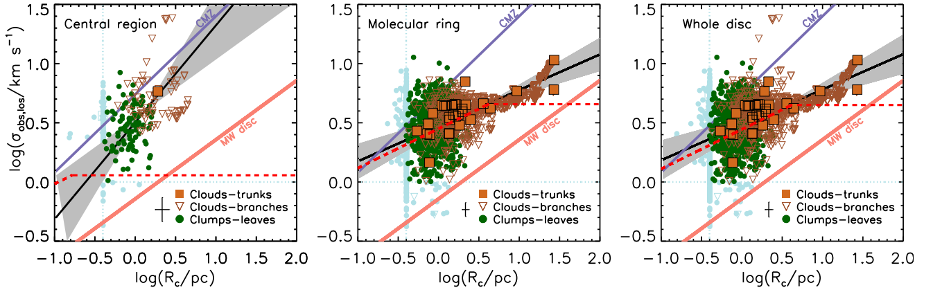
Figure 4. Size – linewidth relation of the molecular structures in the central region, molecular ring and whole disc of NGC 404, respectively. Resolved clumps, i.e. leaves, are shown as filled green circled and resolved clouds, i.e. branches and trunks, are shown as open brown triangles and filled brown squares, respectively. Blue symbols denote unresolved structures. The horizontal and vertical blue dotted lines indicate our resolution limit of 1 \text{ km s}^{-1} (i.e. half the channel width) and 0.40 \text{ pc} (i.e. half the synthesised beam), respectively. In each panel, the black solid line with associated shading shows the best-fitting power-law relation of all resolved molecular structures with 1 \sigma confidence intervals, while the red dashed line shows the R_c - \sigma_{\text{obs,los}} relation predicted by our cloud-cloud collision model (see Section 4.4). The peach and purple solid lines show the size – linewidth relation of the MW disc (Solomon et al. 1987) and MW central molecular zone (Kauffmann et al. 2017), respectively. The typical uncertainty is shown as a black cross to the left of the legend in the bottom-right corner of each panel.
