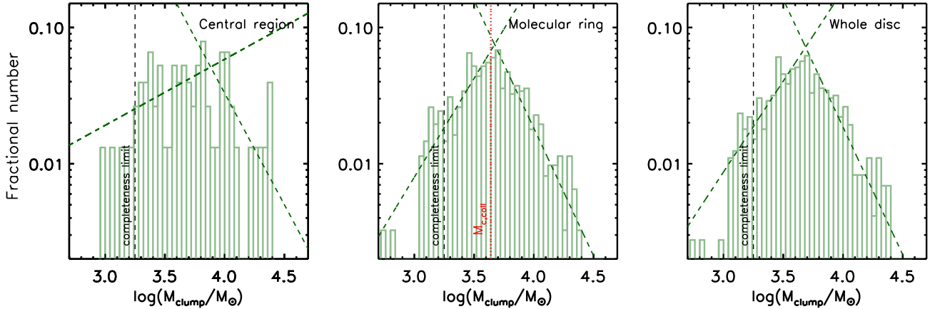
Figure 3. Normalised differential mass distribution function of the resolved clumps in the central region, molecular ring and whole disc of NGC 404, respectively. The two power-laws best fitting the differential mass distribution are overlaid as green dashed lines in each panel. Our mass completeness limit is indicated by a black vertical dashed line in each panel. The red dotted line in the middle panel indicates our model-predicted turn-over mass in the molecular ring ( M_{c,\text{coll}} ; see Sections 4.2 and 6.1 for more details).
