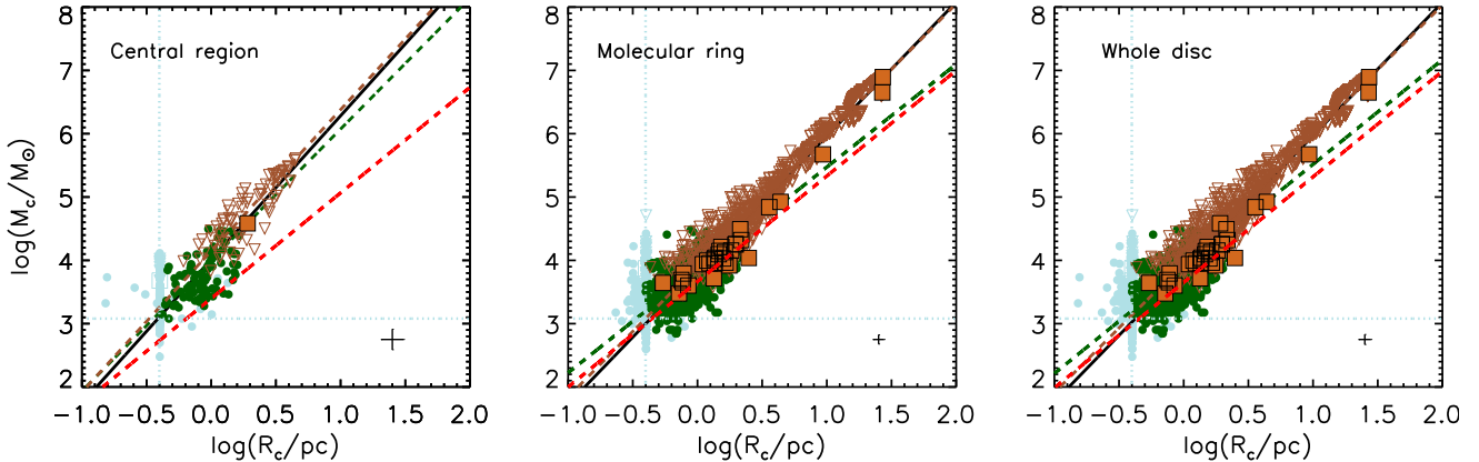
Figure 5. Mass – size relation of the molecular structures in the central region, molecular ring and whole disc of NGC 404, respectively. Symbols are as for Fig. 4. The vertical blue dotted line indicates our spatial resolution limit of 0.40 pc (i.e. half the synthesised beam), while the horizontal blue dotted line indicates our mass detection limit ( \log(10\delta_M/M_\odot) = 3.08 ; see Section 3.1). In each panel, the solid black, green and brown lines show the best-fitting power-law relation of all resolved molecular structures, only resolved clumps (i.e. leaves) and only resolved clouds (i.e. branches and trunks), respectively, while the red dashed line shows the M_c - R_c relation of clumps predicted by our cloud-cloud collision model (see Eq. 35 and Section 5.2).
