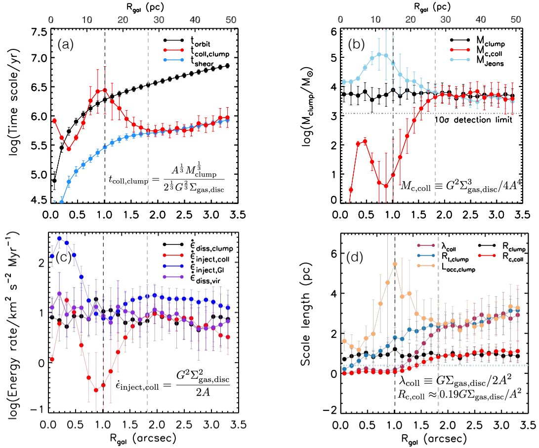
Figure 9. Radial variation of the predicted collision timescale ( t_{\text{coll,clump}} ), clump mass ( M_{\text{c,clump}} ), turbulence energy injection rate ( \dot{\epsilon}_{\text{inject,clump}} ) and clump size ( R_{\text{c,clump}} ), respectively, of our clump-clump collision model, averaged over galactocentric radius bins of 2 pc in NGC 404. In each panel, the black vertical dashed line indicates the boundary ( R_{\text{gal}} = 15 pc) between the central region and molecular ring, while the grey vertical dashed line indicates the galactocentric distance ( R_{\text{gal}} = 27 pc) beyond which the molecular gas disc is no longer gravitationally stable (i.e. Toomre parameter's Q \leq 1 at R_{\text{gal}} \geq 27 pc; see Section 4.5). The error bars of each quantity indicate the 1\sigma scatter of the values within each radial bin (not the uncertainty on the mean within each bin, that is much smaller). Panel (a): comparisons of the orbital timescale t_{\text{orbit}} (Eq. 11), our model-predicted clump-clump collision timescale t_{\text{coll,clump}} (Eq. 6) and the shear timescale t_{\text{shear}} (Eq. 9) at each galactocentric radius. The clump-clump collision timescale t_{\text{coll,clump}} is much smaller than the orbital timescale t_{\text{orbit}} but is in good agreement with the shear timescale t_{\text{shear}} in the molecular ring (especially at R_{\text{gal}} \geq 27 pc where Q \leq 1 ; see Section 4.2). Panel (b): comparisons of the observed median clump mass M_{\text{clump}} , that also happens to be the most common clump mass, our model-predicted clump mass M_{\text{c,clump}} (Eq. 10) and the Jeans mass M_{\text{Jeans}} (Eq. 25) at each galactocentric radius. The black horizontal dotted line indicates our mass detection limit ( \log(10\delta_{\text{M}}/M_{\odot}) = 3.08 ; see Section 3.1). The median/most common clump mass M_{\text{clump}} is in good agreement with the predicted clump mass M_{\text{c,clump}} (and the Jeans mass M_{\text{Jeans}} ) in the molecular ring (especially at R_{\text{gal}} \geq 27 pc where Q \leq 1 ; see Section 4.2). Panel (c): comparisons of the observed median energy dissipation rate (per unit mass) of clumps \dot{\epsilon}_{\text{diss,clump}} (Eq. 14), our model-predicted energy injection rate (per unit mass) due to clump-clump collisions \dot{\epsilon}_{\text{inject,clump}} (Eq. 13), the predicted energy injection rate (per unit mass) from gravitational instabilities \dot{\epsilon}_{\text{inject,GI}} (Eq. 28) and the median virial energy dissipation rate (per unit mass) of clumps \dot{\epsilon}_{\text{diss,vir}} (Eq. 33) at each galactocentric radius. The observed median energy dissipation rate \dot{\epsilon}_{\text{diss,clump}} is consistent with the median virial energy dissipation rate \dot{\epsilon}_{\text{diss,vir}} at all radii, but it agrees well with our predicted energy injection rate \dot{\epsilon}_{\text{inject,clump}} and is within one order of magnitude of \dot{\epsilon}_{\text{inject,GI}} in the molecular ring only (especially at R_{\text{gal}} \geq 27 pc where Q \leq 1 ; see Section 4.4). Panel (d): comparison of the observed median clump size R_{\text{clump}} , that also happens to be the most common clump size, and our model-predicted clump size R_{\text{c,clump}} (Eq. 36), and comparisons of the observed clump tidal radius R_{\text{t,clump}} (Eq. B3), accumulation length L_{\text{acc,clump}} (Eq. 7) and collision critical length \lambda_{\text{coll}} (Eq. 8) at each galactocentric radius. The blue horizontal dotted line indicates our spatial resolution limit of 0''.027 or 0.40 pc (i.e. half the synthesised beam). The clump tidal radius R_{\text{t,clump}} , accumulation length L_{\text{acc,clump}} and collision critical length \lambda_{\text{coll}} are consistent with each other (see Section 4.2) in the molecular ring (especially at R_{\text{gal}} \geq 27 pc where Q \leq 1 ; see Section 5.2), similarly for the observed clump size R_{\text{clump}} and predicted clump size R_{\text{c,clump}} . The clump collision timescale t_{\text{coll,clump}} , tidal radius R_{\text{t,clump}} and accumulation length L_{\text{acc,clump}} are calculated using the median clump mass M_{\text{clump}} at each galactocentric radius (see panel (b)). The quantities t_{\text{coll,clump}} , M_{\text{clump}} , \dot{\epsilon}_{\text{diss,clump}} , \dot{\epsilon}_{\text{diss,vir}} , R_{\text{clump}} , R_{\text{t,clump}} and L_{\text{acc,clump}} are calculated for resolved clumps only.
