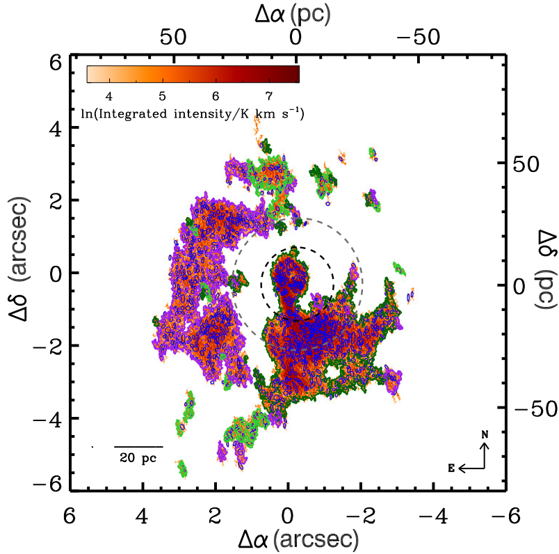
Figure 2. CO(2-1) integrated-intensity map of NGC 404 (colour scale), blanking out faint areas using the CPROPS T00 -generated mask. The mask covers pixels with connected emission above 1.5 \sigma_{\text{rms}} and at least one channel above 3 \sigma_{\text{rms}} , where \sigma_{\text{rms}} is the RMS noise of the data cube. Coloured contours show resolved trunks while blue ellipses show resolved leaves (i.e. clumps; extrapolated to the limit of perfect sensitivity but not corrected for the finite angular resolution). The black dashed ellipse at a galactocentric distance of 15 pc separates the central region and molecular ring discussed in the text, while the grey dashed ellipse at a galactocentric distance of 27 pc indicates the galactocentric distance beyond which the molecular gas disc is no longer gravitationally stable (i.e. the Toomre parameter Q \leq 1 at R_{\text{gal}} \geq 27 pc; see Section 4.5 for more details). The synthesised beam ( \approx 0''.058 \times 0''.034 or \approx 0.86 \times 0.51 pc 2 ) is shown as a very small black ellipse to the left of the scale bar in the bottom-left corner.
