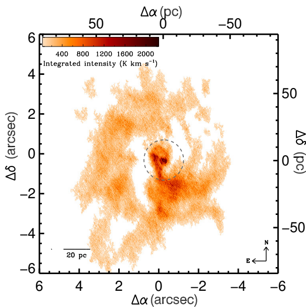
Figure 1. Moment-zero map of the ^{12}\text{CO}(2-1) emission of NGC 404 derived from our ALMA observations. The synthesised beam ( \approx 0''.058 \times 0''.034 or \approx 0.86 \times 0.51 \text{ pc}^2 ) is shown as a very small black ellipse to the left of the scale bar in the bottom-left corner. The grey dashed ellipse at a galactocentric distance of 15 pc separates the central region and molecular ring discussed in the text.
