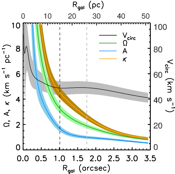
Figure B1. Galactocentric distance dependence of the orbital circular velocity V_{\text{circ}} (black curve), orbital circular angular velocity \Omega (green curve), Oort’s constants A (blue curve) and epicyclic frequency \kappa (orange curve) in NGC 404. The coloured envelope around each curve indicates the \pm 1 \sigma uncertainties. The black vertical dashed line indicates the boundary ( R_{\text{gal}} = 15 pc) between the central region and molecular ring, while the grey vertical dashed line indicates the galactocentric distance ( R_{\text{gal}} = 27 pc) beyond which the molecular gas disc is no longer gravitationally stable (i.e. Toomre parameter’s Q \leq 1 at R_{\text{gal}} \geq 27 pc; see Section 4.5). The circular velocity curve is nearly flat in the molecular ring.
