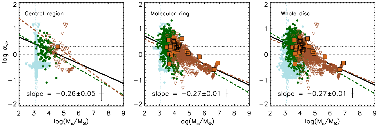
Figure 7. Virial parameter – gaseous mass relation of molecular structures in the central region, molecular ring and whole disc of NGC 404, respectively. Symbols are as for Fig. 4. The black dashed lines indicate \alpha_{\text{vir},c} = 1 and the black dotted lines \alpha_{\text{vir},c} = 2 , above which structures are unbound in the absence of other confining mechanisms. In each panel, the black, green and brown lines show the best-fitting power-law relation of all resolved molecular structures, only resolved clumps (i.e. leaves) and only resolved clouds (i.e. branches and trunks), respectively. The slope of the best-fitting power-law relation of all resolved molecular structures is listed in the legend. The vertical blue dotted lines indicate our mass detection limit ( \log(10\delta_M/M_{\odot}) = 3.08 ; see Section 3.1).
