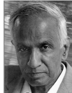
S. Chandrasekhar, 1910 - 1995
