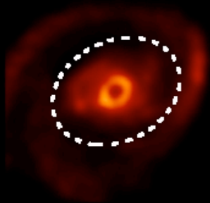
NGC 4736
