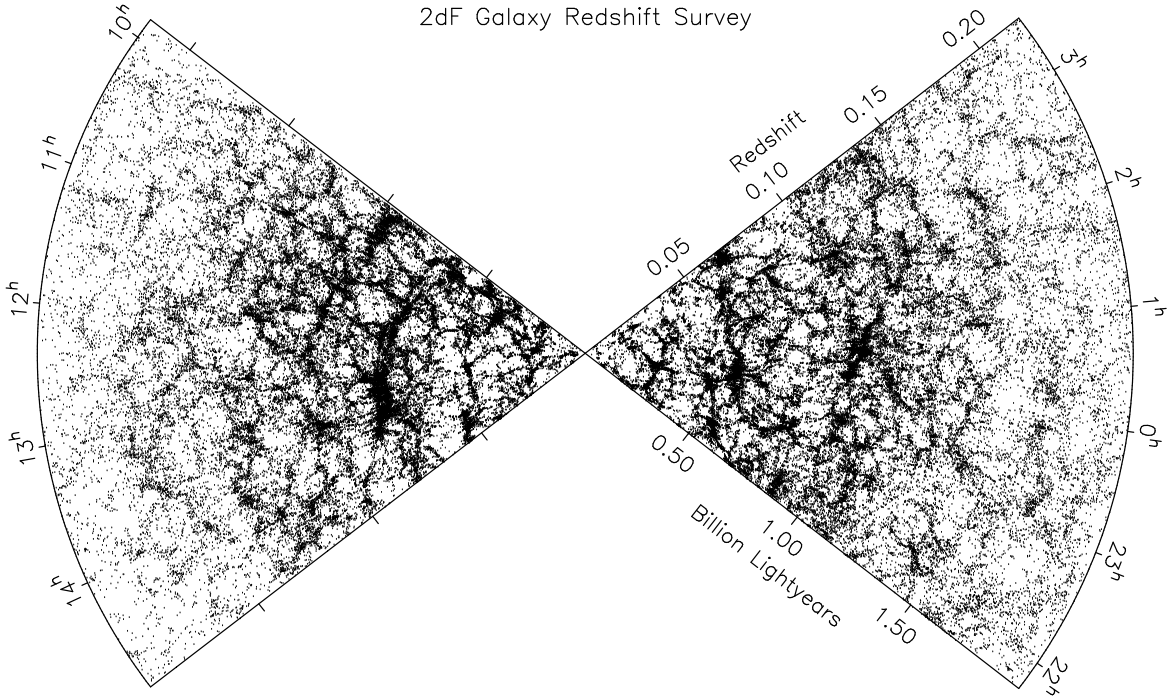
Figure 2: A survey of galaxies over the sky illustrates there are inhomogeneities spanning a wide range of scales (2dF Galaxy Redshift Survey -based at Oxford)
