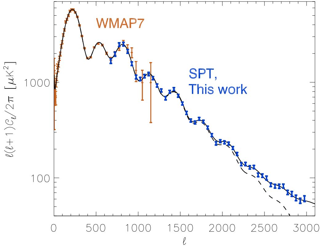
Figure 5: The best fit power spectrum of the CMB as compared to the WMAP and SPT data (Keisler 2011)
