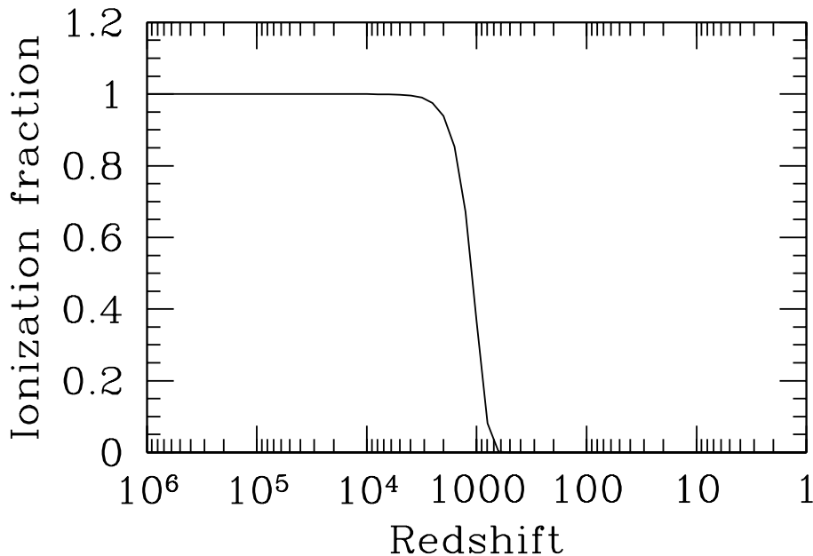
Figure 4: The evolution of the ionization fraction as a function of redshift
