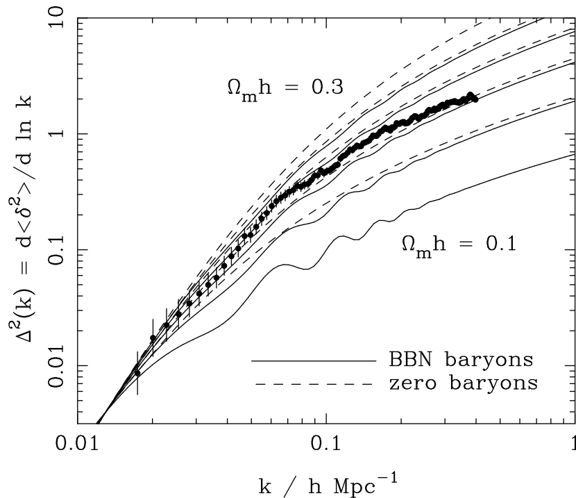
Figure 3: The mass variance, \Delta^2(k) of inhomogeneities with cold dark matter compared to the real universe
