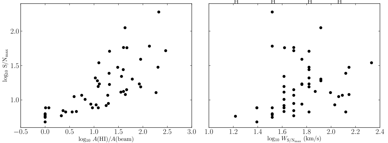
Figure 6. Peak signal to noise (S/N)_{\max} of all galaxies detected in the standard, 12-h HI cubes (see text) plotted against the size of the HI system in units of the beam (left), and the spectral line width at the position of (S/N)_{\max} (right). The top H symbols represent the FWHM of the Hanning filters used to smooth the HI cubes when searching for emission (see Sec. 3).
