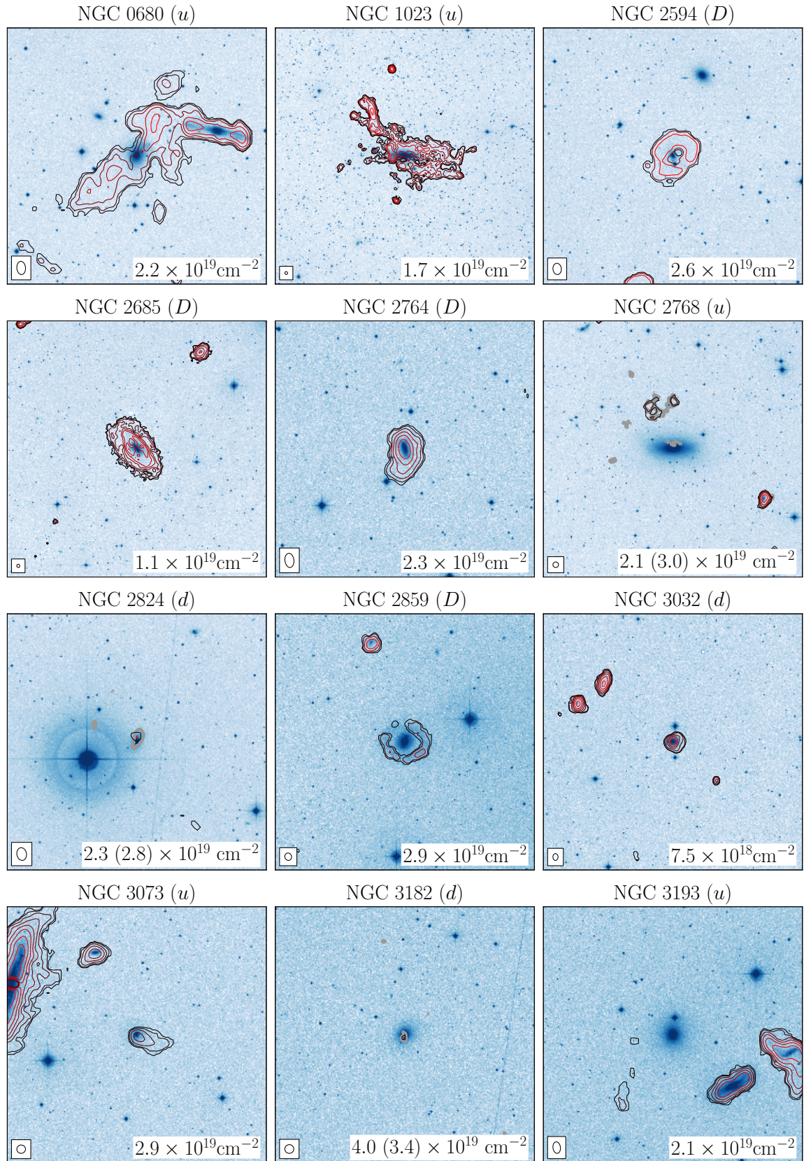
Figure A1. Total-H I contours on top of DSS images of all H I-detected galaxies. Images are centred on the target galaxy and show a fixed area of 180 \times 180 \text{ kpc}^2 at the galaxy distance. Contour levels are N(\text{H I})=N_0 \times 2^n with N_0 given at the bottom of each image and n = 0, 1, 2, \dots . Contours are coloured black to red, faint to bright. The beam is shown on the bottom left. In the cases where the R01 image reveals H I missing from the standard image we show its lowest contour with a thick grey line (contour level in parenthesis).
