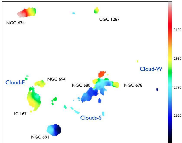
Figure 12. Velocity map of the HI emission in the NGC 680 group of galaxies. The intensity scale in \text{km s}^{-1} is shown to the right. The field of view is 0.8 \times 0.7 degree.
