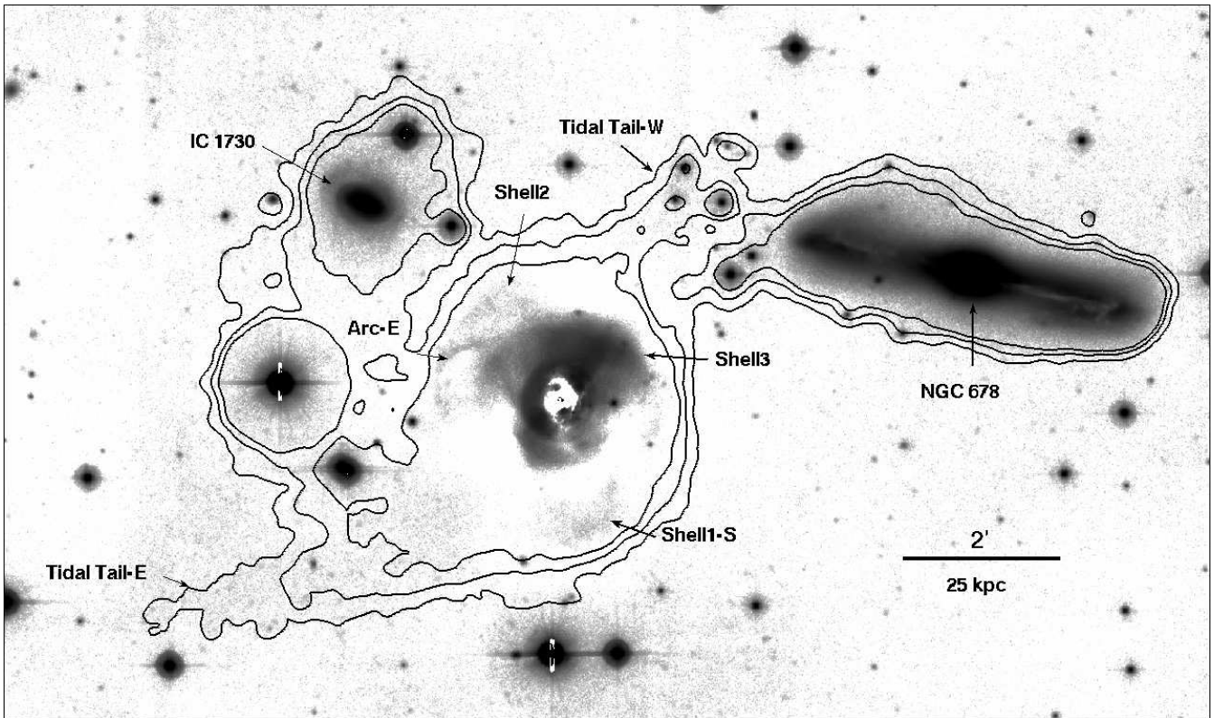
Figure 4. g-band surface brightness map of NGC 680, after the subtraction of a galaxy model with a single Sersic index of 4. The faint foreground stars and distant background galaxies have been subtracted from the image. The contours of the galactic emission before the galaxy subtraction, as shown on Fig. 3, are superimposed (levels: 28, 27 and 26 \text{ mag arcsec}^{-2} ). The various fine structures disclosed by the image are labeled.
