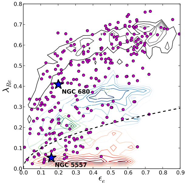
Figure 14. Position of NGC 680 and NGC 5557 in the \lambda_{Re} vs \epsilon_e diagram. The dots represent the ATLAS 3D ETGs. The contours the distribution of simulated merger remnants for slow (red), fast (blue) rotators, remergers (green) and progenitors (black). Figure adapted from Paper VI.
