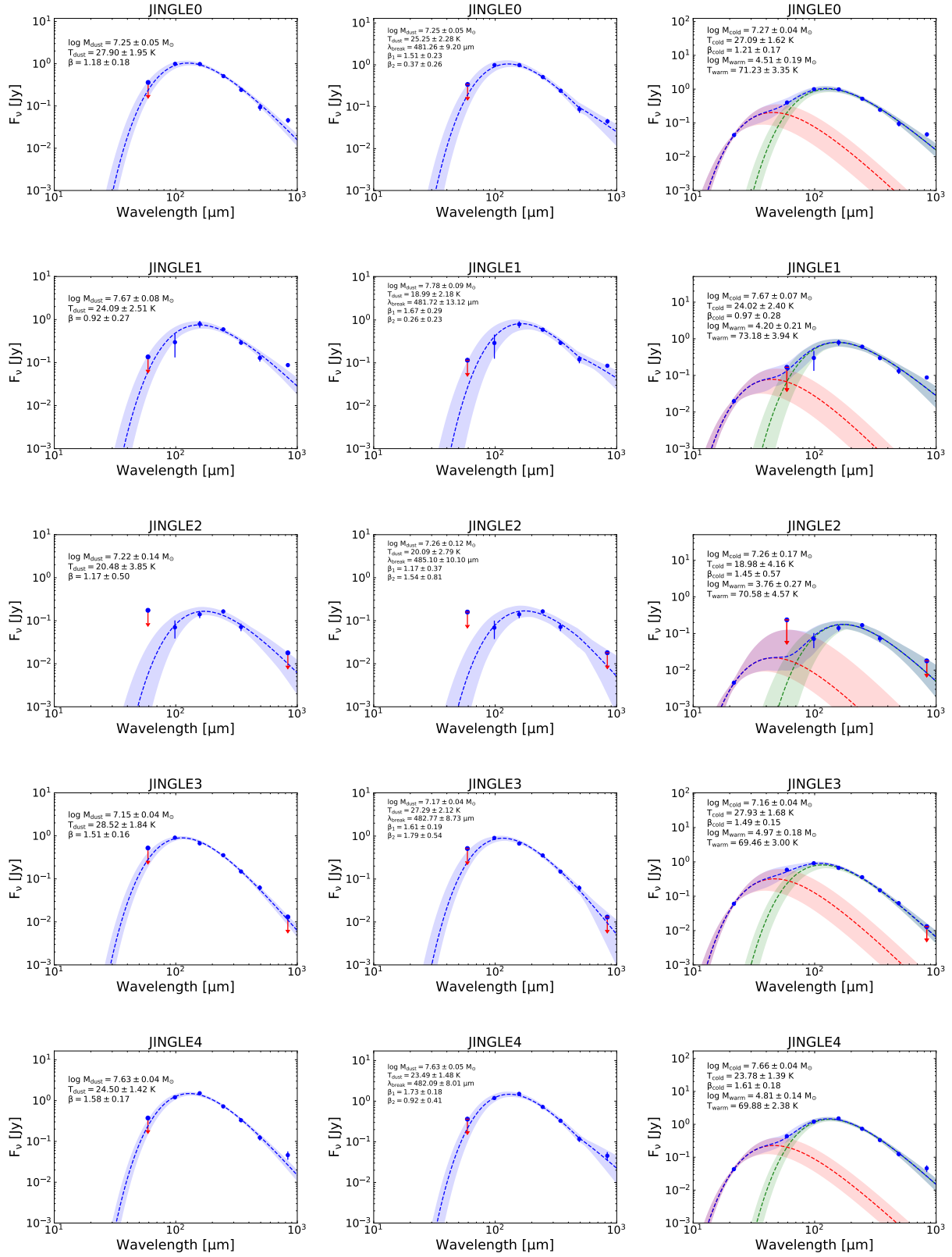
Figure D2. FIR SED of the galaxies of the JINGLE sample, fitted with the hierarchical approach using the three models: SMBB (left panel), BMBB (middle panel) and TMBB (right panel). The shaded regions show the lower and upper 1-sigma uncertainties on the SED models, defined by taking the maximum and minimum flux values of the models with likelihood values in the highest 68th percentile. Additional figures showing the entire sample of 192 JINGLE galaxies are available online.
