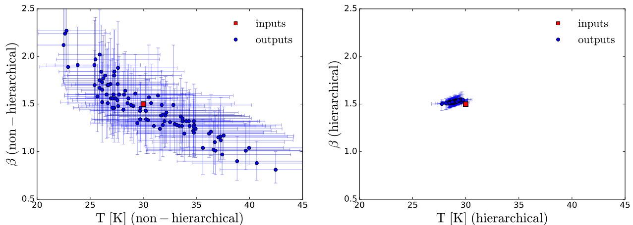
Figure 3. Results of temperature and \beta from the fit of 100 simulated SMBB SEDs with the same input parameters ( \log M_{dust} = 8 M_{\odot} , T = 30 K, and \beta = 1.5 ) and 10% added noise. The output values are derived with the non-hierarchical (left panel) and hierarchical (right panel) SED fitting method. In red is shown the input value and in blue are the measured values.
