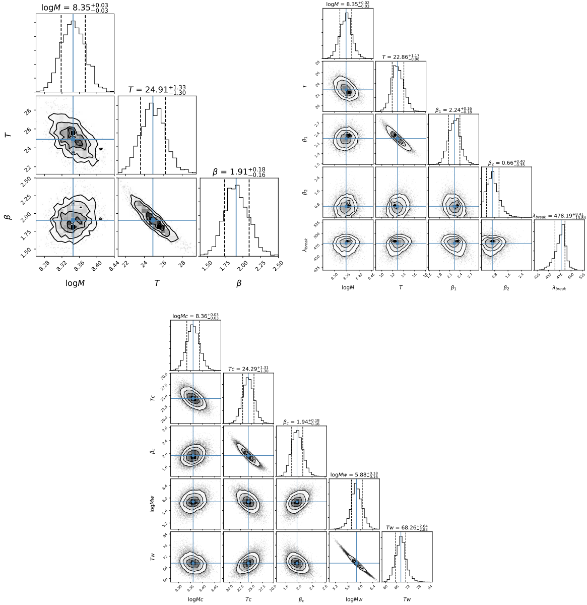
Figure D1. Example of the posterior probability density functions (PDFs) of the model parameters obtained using the hierarchical method for the fit of one galaxy (JINGLE 147). The three panels show the results of fit using the SMBB (upper left), BMBB (upper right) and TMBB (bottom) models. The blue line indicates the median values, the dotted lines show the 16th and 84th percentiles, that indicate the one-sigma uncertainties on the parameters.
