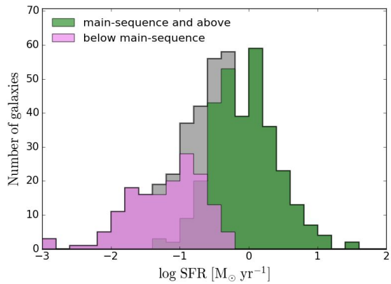
Figure 2: Comparison of the results of the SED fit of the two sub-samples (“main-sequence” and “below main-sequence”) fitted together or separately:
