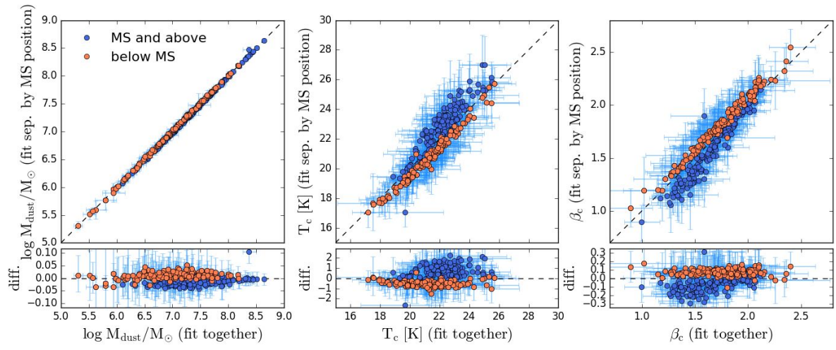
Figure 2: Comparison of the results of the SED fit of the two sub-samples (“main-sequence” and “below main-sequence”) fitted together or separately:
