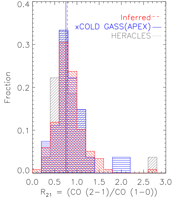
Figure 9. Distribution of CO(2-1)-to-CO(1-0) line ratios for the inferred (based on observed L_{\text{CO}(2-1)} and predicted L_{\text{CO}(1-0)} ) and observed (literature) samples. The red histogram shows the inferred R_{21} , while the blue and gray histograms show the observed xCOLD GASS (with APEX) and HERACLES survey, respectively. The colored vertical lines indicate the median R_{21} of each sample.
