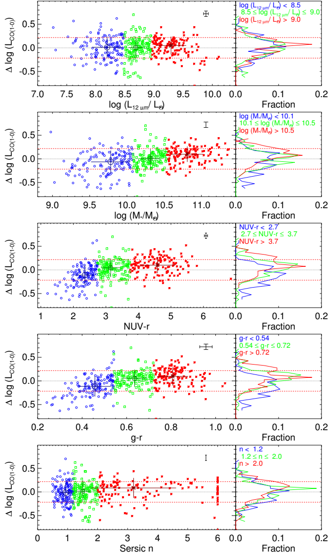
Figure 5. In the left-hand panels, for CO(1-0) detections, we plot the residuals ( \Delta \log(L_{\text{CO}(1-0)}) \equiv \log(L_{\text{CO}(1-0),\text{obs}}) - \log(L_{\text{CO}(1-0),\text{est}}) ) of CO(1-0) luminosity predicted from the best-fitting relation (Eq. 3) between L_{\text{CO}(1-0)} and L_{12\mu\text{m}} and the observed L_{\text{CO}(1-0)} as a function of 12\mu\text{m} luminosity L_{12\mu\text{m}} , stellar mass M_* , NUV- r color, g-r color and Sersic index n (from top to bottom). The dashed red horizontal lines show the 1\sigma total/observed scatter of all galaxies, and the characteristic error bars illustrate the median value of available measurement uncertainties. In each panel, we divide the galaxies into 3 sub-samples (with the same number of galaxies in each) according to the parameter considered. Blue circles, green squares and red stars correspond to respectively the smallest, intermediate and largest parameter values, and the large symbols show the median and scatter in each bin. In the right-hand panels, the different colors show the distribution of the residuals in each sub-sample.
