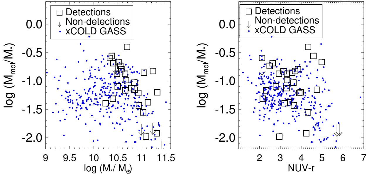
Figure 10. Distribution of our sample galaxies on the planes of molecular-to-stellar mass ratio \log(M_{\text{mol}}/M_*) versus \log(M_*) (middle) and \log(M_{\text{mol}}/M_*) versus \text{NUV-r} (right). In each panel, our galaxies are plotted as large symbols (black squares for CO detections and downward-pointing arrows for upper limits), while the detections from the xCOLD GASS survey are plotted as blue dots.
