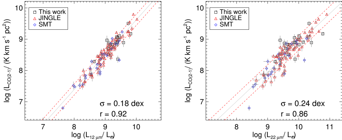
Figure 4. As Figure 3, but for the CO(2-1) luminosities.
