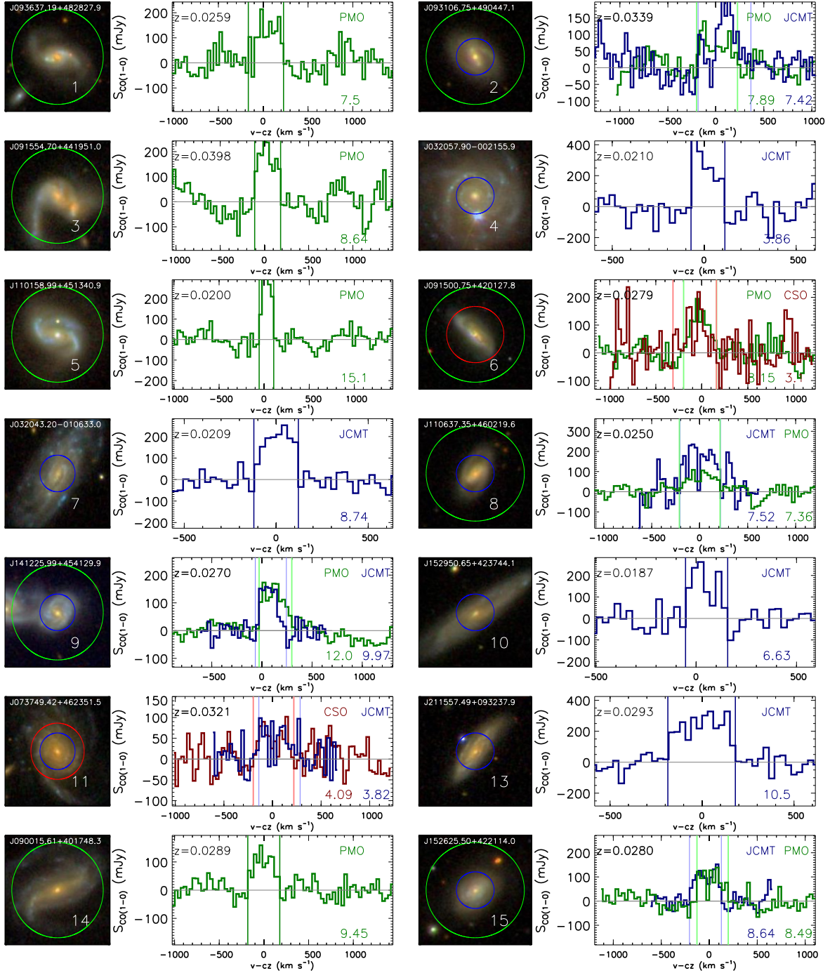
Figure 2. SDSS color images and CO spectra of our target galaxies. Each galaxy’s SDSS name and target number are overlaid on each image, while the telescope used and the S/N are noted in the top-right and bottom-right corner of each spectrum. The green, blue and red circles overlaid on the images show the beam size of respectively PMO, JCMT and CSO as relevant. We used PMO to observe CO(1-0) and JCMT and CSO to observe CO(2-1). To directly compare the intensities from different telescopes, all spectra are in S_{\text{CO}(1-0)} units (assuming R_{21} = 0.7 ) and binned into channels \sim 30 \text{ km s}^{-1} wide.
