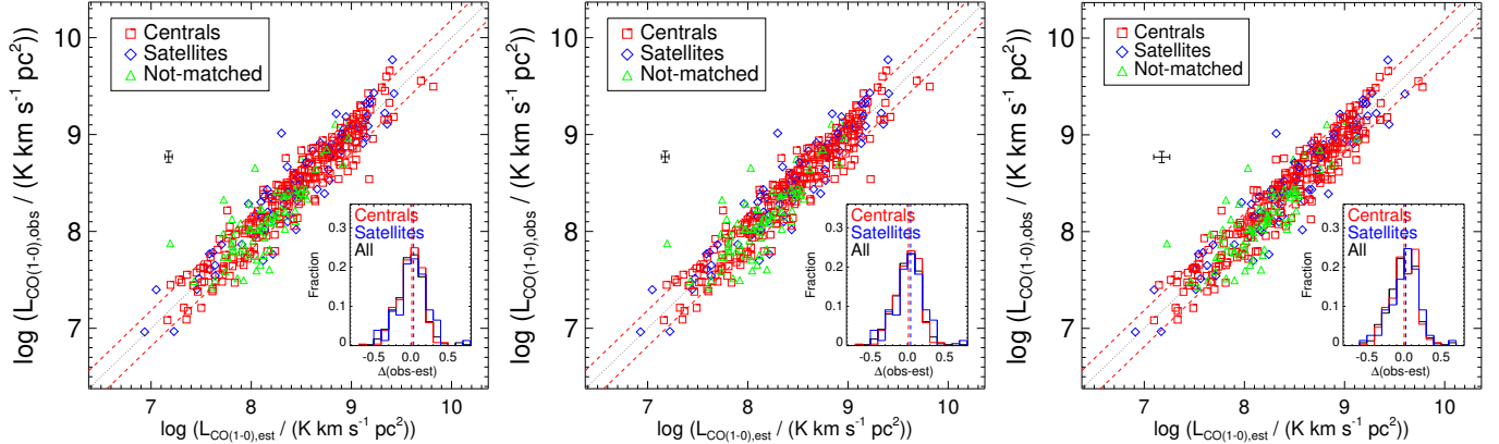
Figure 8. As Figure 7 but for alternative estimators of the CO(1-0) luminosity ( L_{\text{CO}(1-0)} ) based on L_{12\mu\text{m}} , g-r color and r -band luminosity (left); L_{12\mu\text{m}} , g-r color and z -band luminosity (center); L_{12\mu\text{m}} , r - and z -band luminosities (right). The characteristic error bars shown illustrate the median (direct or derived) measurement uncertainties.
