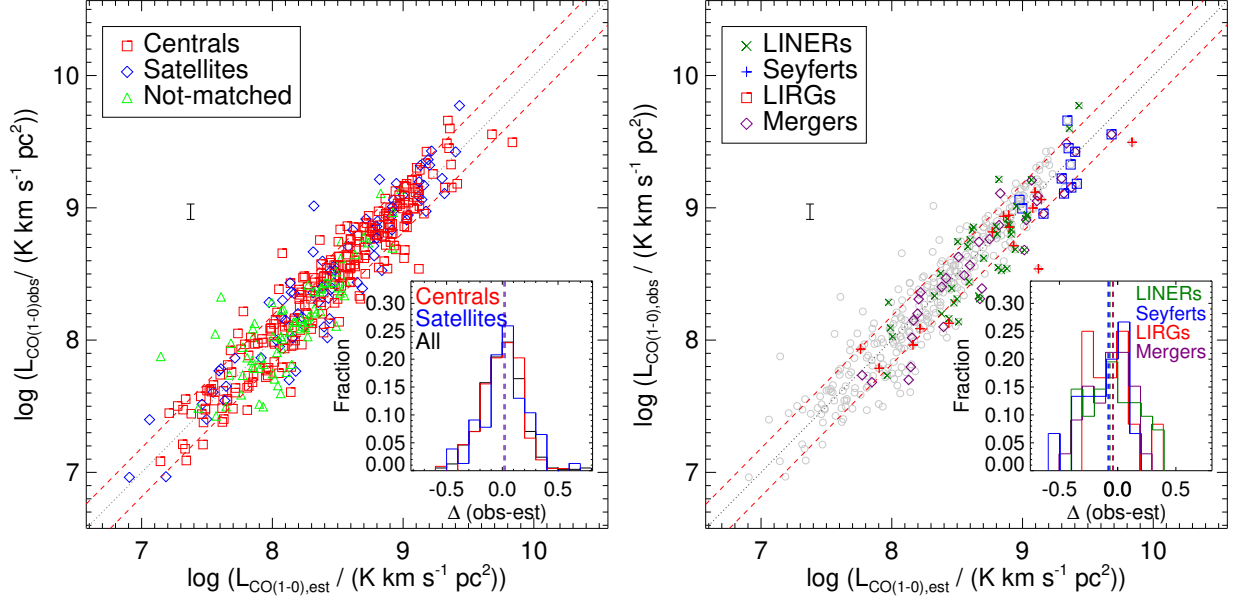
Figure 7. New estimator of the CO(1-0) luminosity ( L_{\text{CO}(1-0)} ) based on L_{12\mu\text{m}} , M_* and g-r , as well as the distribution of the residuals of some sub-samples. In each panel, the dotted black line and two dashed red lines show respectively the best-fitting relation (with parameters listed in Table 4) and the 1\sigma total/observed scatter (0.18 dex) of all galaxies. In the left panel, different symbols/colors are used to highlight any difference between central and satellite galaxies. In the right panel, we highlight particular galaxy populations including BPT-selected AGN hosts (LINERs as dark green crosses and Seyferts as blue plus signs), LIRGs (red squares) and interacting galaxies or mergers (purple diamonds). In insets, the histograms and vertical dashed lines show respectively the distributions and median values of the residuals for different sub-samples.
