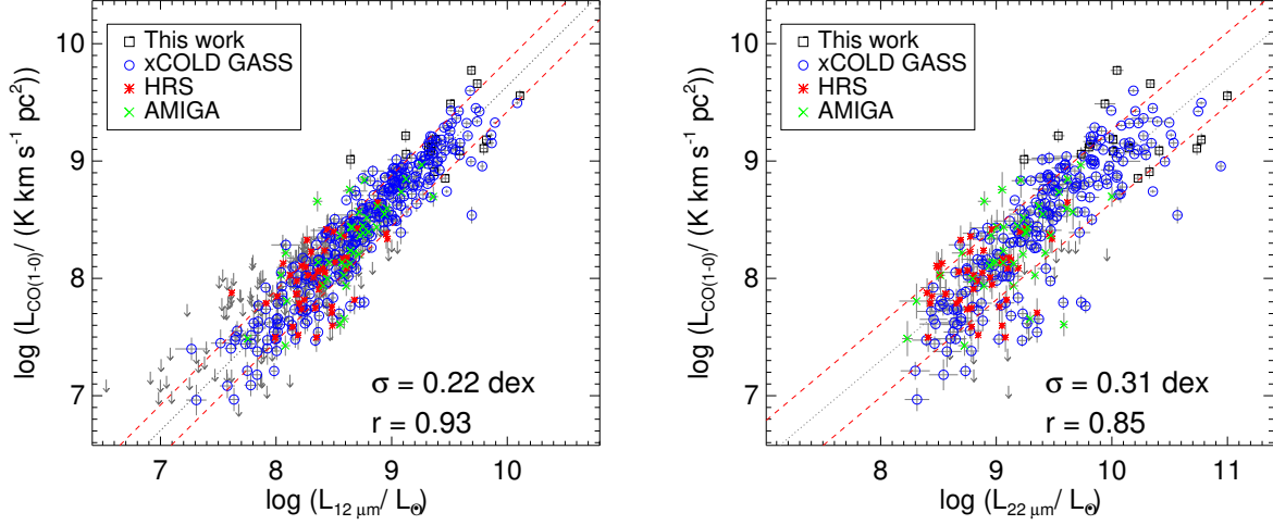
Figure 3. Correlation of the CO(1-0) luminosities with the mid-infrared luminosities from WISE measured in the 12 (left panel) and 22 \mu\text{m} (right panel) band. Different colors/symbols indicate detections in different CO samples, as indicated in the top-left corner of each panel, and the grey error bars to show their measurement uncertainties, while the dark grey downward-pointing arrows mean upper limits from xCOLD GASS. In each panel, the dotted black line and two dashed red lines show respectively the best-fitting linear relation (with parameters listed in Table 3) and the 1\sigma total/observed scatter for detections only obtained from all the samples together. The total/observed scatter ( \sigma ) and the Spearman's correlation coefficient ( r ) for all the detections are listed in the bottom-right corner of each panel.
