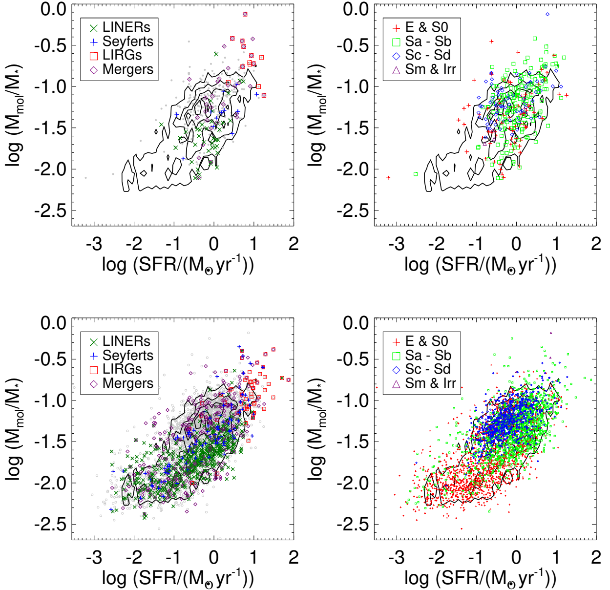
Figure 11. Distribution of galaxies on the plane of molecular gas-to-stellar mass ratio versus star formation rate. The upper panels show the distribution of our sample and xCOLD GASS with observed gas masses, and the lower panels show the distribution of the MaNGA/MPL-8 sample for which the gas masses are estimated using our three-parameter L_{\text{CO}(1-0)} estimator (Eq. 4). Different colors/symbols represent different types of galaxies (left) or different morphologies (right), as indicated. Black contours show the distribution of the whole MaNGA/MPL-8 sample, repeated in every panel for comparison.
