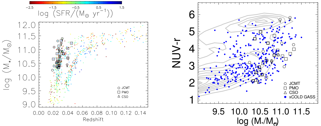
Figure 1. Distribution of our target galaxies on the plane of stellar mass versus redshift (left panel) and the plane of NUV- r color versus stellar mass (right panel). In both panels, the open circles, squares and triangles represent our targets that are observed with the JCMT, PMO and CSO respectively. Symbols with a downward arrow represent CO upper limits from our JCMT observations. Small filled circles in the left panel show the MaNGA MPL-3 sample for comparison, color-coded by star formation rate taken from Salim et al. (2016) . Blue dots in the right panel show CO detections from the xCOLD GASS survey, while the grey contours show the distribution of a volume-limited galaxy sample selected from the SDSS/DR7 main galaxy sample.
