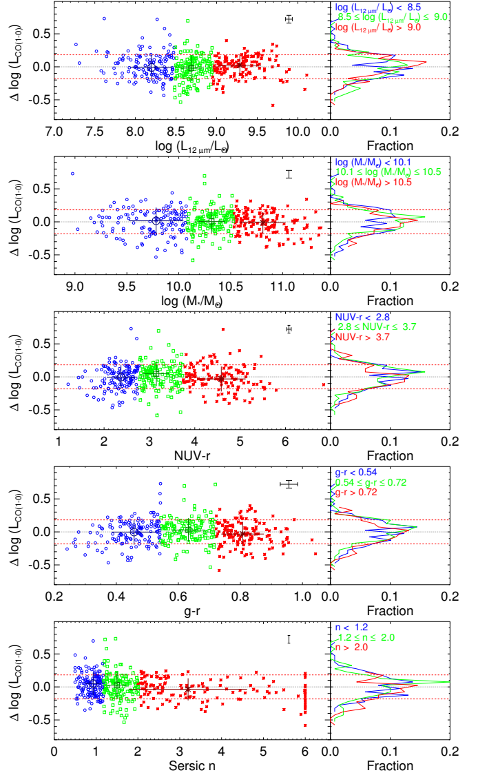
Figure 6. As Figure 5 but for the residuals of the predicted value of L_{\text{CO}(1-0)} using the three-parameter estimator (Eq. 4).
