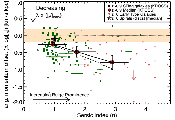
Figure 9. Specific angular momentum offset (see Section 4.3.1) as a function of Sérsic index for the KROSS sample and z=0 early-type galaxies. The large data points show the running median and bootstrap errors. The dashed line shows the same running median but using j_{n=0} for all galaxies (see Section 4.3). The shaded region represents the 0.2 dex scatter expected for the distribution of halo spins, \lambda . The downward arrow represents the median systematic offset to apply to the z=0 early-type galaxies when using an alternative stellar mass fraction to the disks (see Section 4.3). On average, galaxies with higher Sérsic indices (a proxy for bulge fraction) have lower specific angular momentum at both redshifts.
