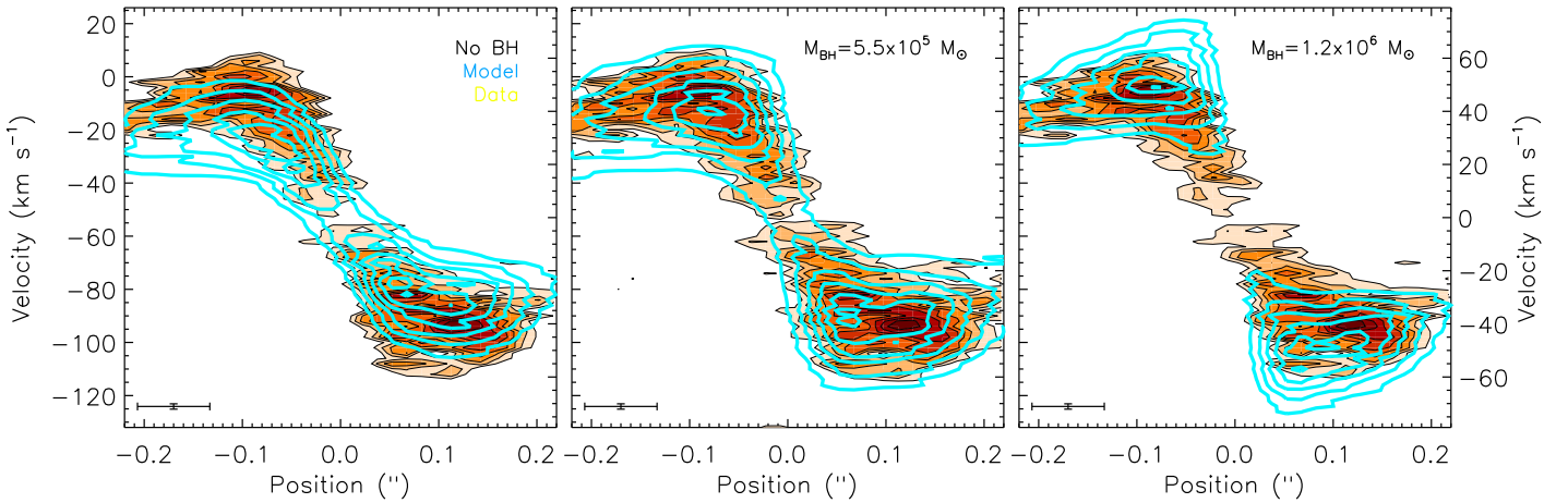
Figure 11. Position-velocity diagram extracted from the observed NGC 404 datacube (orange), overplotted with position-velocity data taken from our KINMS models (blue contours). Our spatial and velocity resolutions are shown as an error bar in the bottom-left corner of each plot. The central panel shows our best-fitting model with a 5.5 \times 10^5 M_{\odot} IMBH, while the left and right panels show the same model with no BH, and with a SMBH ( M_{\text{BH}} = 1.2 \times 10^6 M_{\odot} ), respectively. Clearly our best-fitting model provides a much better fit to the data.
