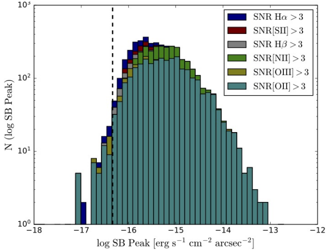
Figure 9. Surface brightness (SB) function of the H II regions in the commissioning data of NGC 628. The black dashed line shows the detection threshold of one element of resolution in H\alpha . The different colors represent selected subsets of regions for which there is a detection of different strong lines (see the legend). The few regions below the black dashed line are faint H\alpha regions detected from the combination of H\alpha , H\beta and [O III]\lambda 5007 used for the identification.
