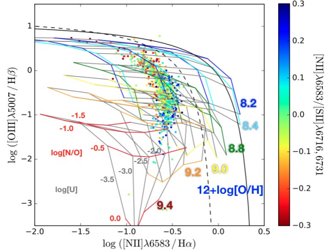
Figure 10. BPT diagram (Baldwin et al. 1981) of emission line regions identified in NGC 628 (from Rousseau-Nepton et al. 2018) along with a grid of models from BOND (Vale Asari et al. 2016) using the SED of a 3 Myr old stellar cluster with a Chabrier IMF (Chabrier 2003). The colors of the grids indicate different metallicities ( 12+\log[O/H] ). Horizontal lines have different values of \log[N/O] , as given in red for 12+\log[O/H]=9.4 , and vertical lines have different values of \log[U] , as given in gray for the same metallicity. The color-scale of the scattered observational points indicates the \log([N II]\lambda 6583/[S II]\lambda 6716, 6731) line ratio which is known to be a good indicator of \log[N/O] (Pérez-Montero et al. 2014). The limit between the H II regions and the transition regime (Kauffmann et al. 2003) is shown by the dashed curve, and the extent of the starburst domain (Kewley et al. 2001), is displayed by the continuous curve.
