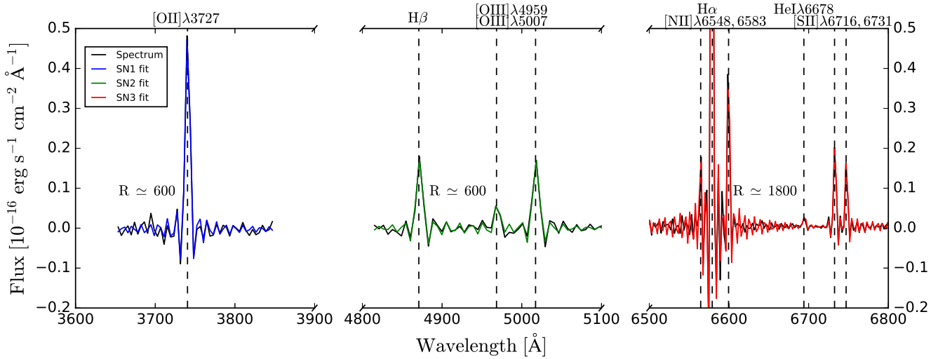
Figure 2. Continuum subtracted spectrum of an H II region in NGC 628 extracted from the datacubes using a circular aperture with a radius of 1.6'' , centered at RA 01h36m53.1s and DEC +15^{\circ}48'04.8'' . The fits obtained with ORCS (Sect. 5) for the emission lines are shown. Note that SITELLE’s line profiles are fitted using a cardinal sine function. Spectral resolutions obtained here are significantly smaller than those selected for SIGNALS.
