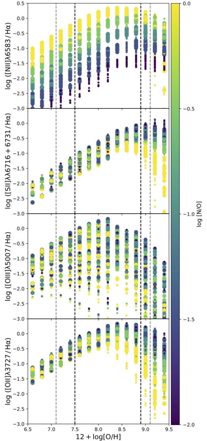
Figure 8. Prediction of several strong line ratios ( [\text{line}]/\text{H}\alpha ) of the CLOUDY photoionization code (extracted from the BOND grid of models on 3MdB). The color scale represents the \log[\text{N}/\text{O}] ratio for a given model. The smaller dots correspond to models representing less expected regions ( \log[\text{N}/\text{O}] < -1.5 or age > 5.1 Myr or \log[\text{U}] \geq -3.55 ). The grey dashed vertical lines show the expected range of metallicity of the regions sampled and the black dashed vertical line shows the usual range of metallicity for most regions in the local Universe.
