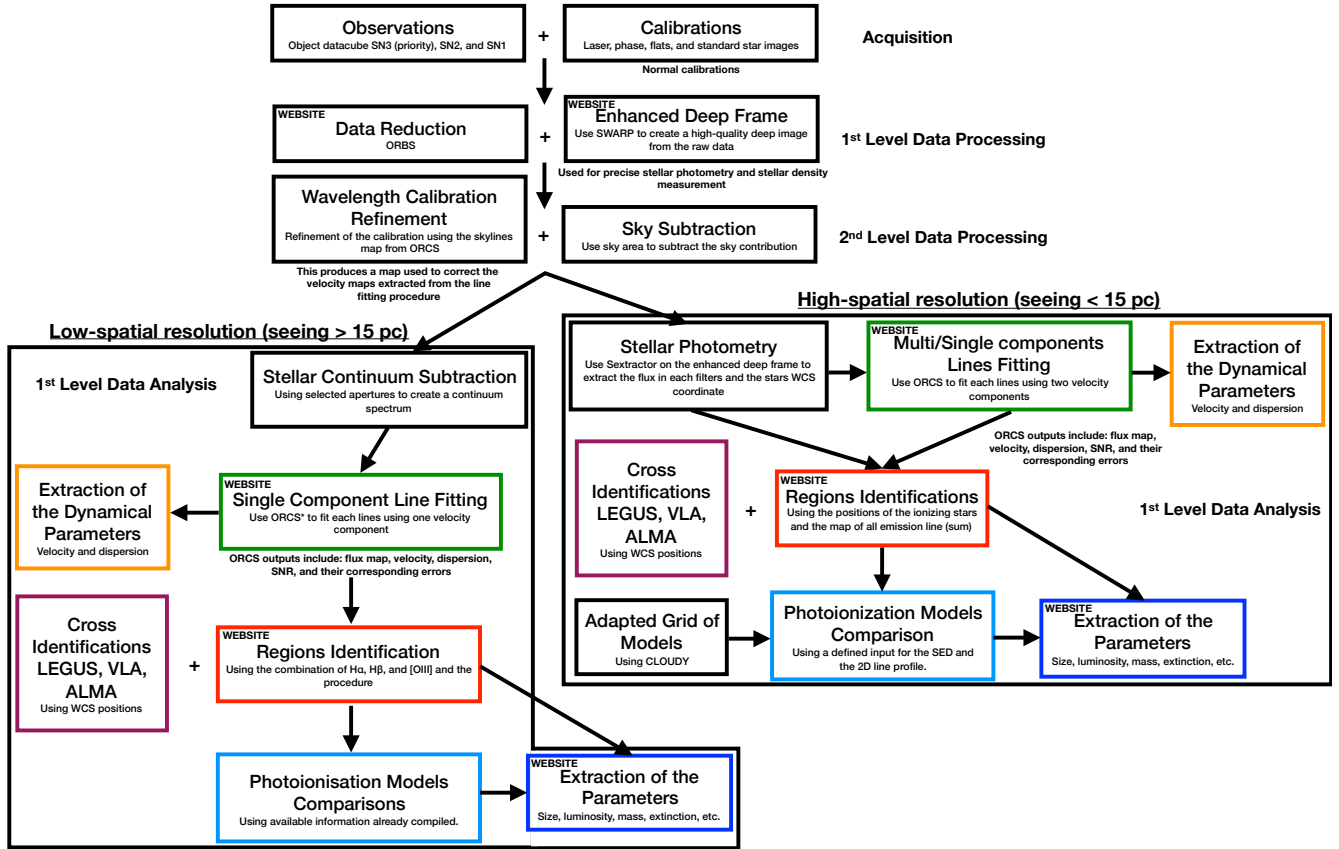
Figure 14. Organizational chart for the data processing. All items with the label WEBSITE will be accessible to everyone via our Website ( http://www.signal-survey.org ) once the collaboration team has analyzed the data and published the different catalogs. Note that all observed datacubes are available at the Canadian Astronomical Database Center (CADC).
