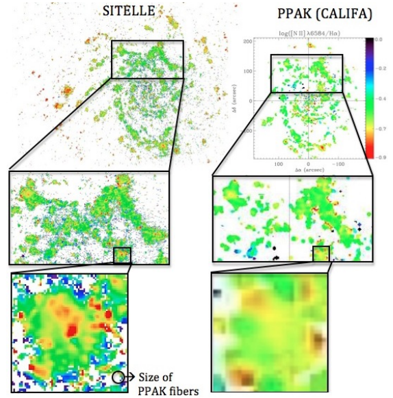
Figure 6. Spatial resolution and filling factor impact on the measurements of emission line ratios. The line ratio \log([\text{N II}]\lambda 6583/H\alpha) extracted from SITELLE’s observations on NGC 628 (0.8” seeing, 0.32” per pixel, 100% filling factor) is compared to PPAK’s observations on the same area (0.8” seeing, 2.7” per fiber, 60% filling factor). The color scale is the same for both maps (upper-right corner). The PPAK map (on the right) is published in Rosales-Ortega et al. (2011) and was re-used here for comparison purpose only.
