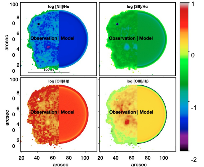
Figure 11. Comparison of a giant H II region observed with SIFELLE in NGC 6822 with a 3D photoionization model projected on 2D images. The region is split in two for each panel: the left side represents the observations while the right side is the model (a slice perpendicular to the line of sight that goes from the center of the region to the outskirts). A pure 40 000 K Planck function was used as ionizing spectrum and abundances at 20% of the solar value, excepted for S. The model was also for a thin shell of gas with \log[U] = -2.6 .
