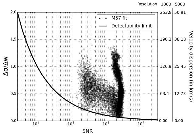
Figure 3. Instrument line spread function ratio. The black line shows the minimum measurable ratio \Delta\sigma (observed) / \Delta\omega (theoretical or pure sinc) for a line with a given SNR. The corresponding velocity dispersion at the two different resolutions used for SIGNALS (5000 and 1000) are reported on the right axis. It scales linearly with the resolution. A set of points from a fit of NGC6720 data with ORCS (Martin & Drissen 2017) is overlapped to the prediction. In this case, we can see that the SNR of the data points is high because all the lines in each spectrum are fitted with the same broadening parameter.
