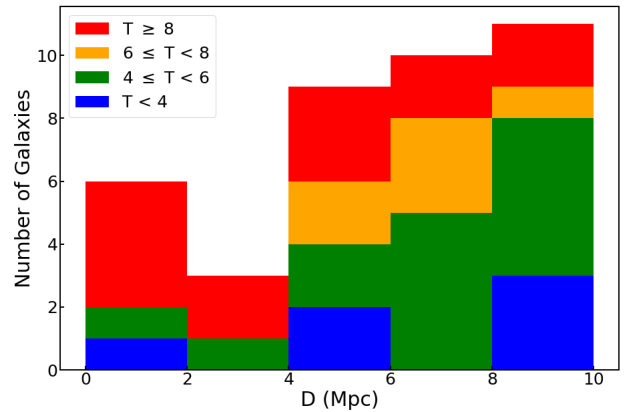
Figure 5. Distribution of the primary targets as a function of distance. The galaxies are color-coded according to their morphological type, as given by the parameter T from the revised Hubble classification scheme.
