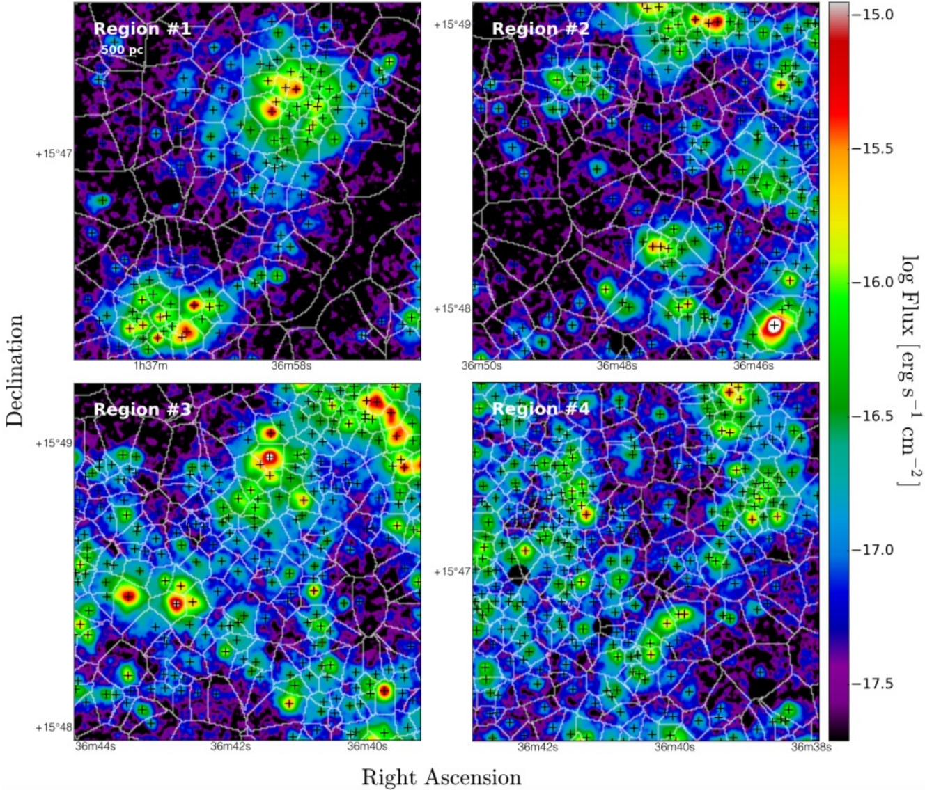
Figure 7. Examples of ionizing sources and their zone of influence in NGC 628 drawn over the \text{H}\alpha + \text{H}\beta + [\text{O III}]\lambda\lambda 4959, 5007 continuum-subtracted image from Rousseau-Nepton et al. (2018). The centroid position of each emission peak detected is identified with a cross. The white contours define the zones of influence surrounding the emission peaks.
