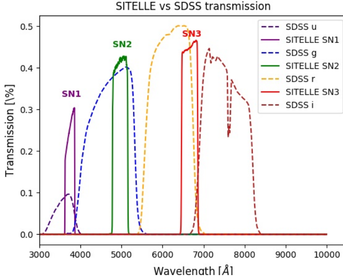
Figure 4. Transmittance curves for the atmospheric (airmass=1), telescope and optical assembly from SITELLE and SDSS. The SIGNALS filters (SN1, SN2, and SN3) are shown along with the overlapping SDSS filters.
