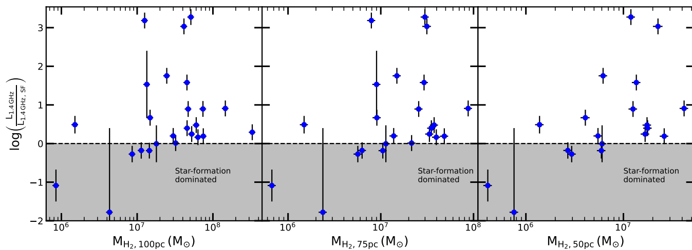
Figure 3. Molecular gas mass within an aperture of a given radius (100, 75 and 50 pc, as indicated by the x-axis labels) versus excess 1.4 GHz radio continuum fraction (after the contribution from star formation has been removed).
