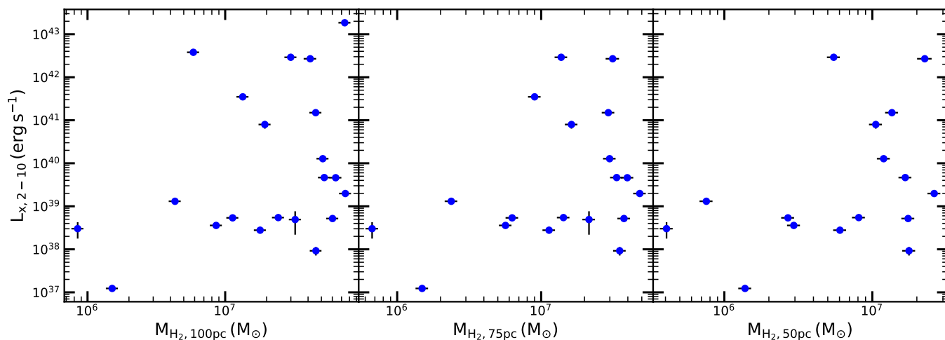
Figure 4. As Figure 3, but for the 2–10 keV X-ray luminosity.
