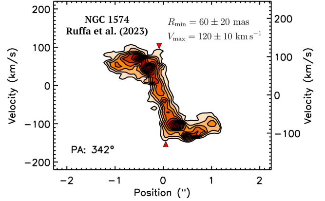
Figure B1. Major-axis position-velocity diagram of the CO(2-1) emission of the galaxy NGC 1574 (Fig. 5d of Ruffa et al. 2023). The red triangles indicate the data points we adopt as the innermost kinematic tracer.
