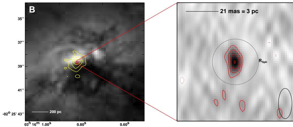
Figure 1. (Left): NGC 1266 Hubble Space Telescope B -band greyscale imaged. CARMA CO(1–0) v_{\text{sys}} contours are overlaid in yellow at levels of [0.25, 0.5, 0.75] of the peak CO emission ( \gtrsim 1937 \text{ K km s}^{-1} ). The box shows the field-of-view of the VLBA image to the right. (Right): NGC 1266 1.65 GHz continuum image with contours. The VLBA beam is the black ellipse in the lower right corner and has a major axis diameter of 9.75 mas (1.14 pc). The relative contour levels are [-3, 3, 6, 10, 14] and the unit of the contour level is 42 \mu\text{Jy beam}^{-1} . The AGN is detected to 14\sigma significance, and the VLBA does indeed probe the sphere of influence ( R_{\text{Sph}} ), but does not appear to resolve the point source.
